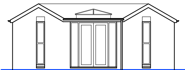
FRONT ELEVATION (1:100)
