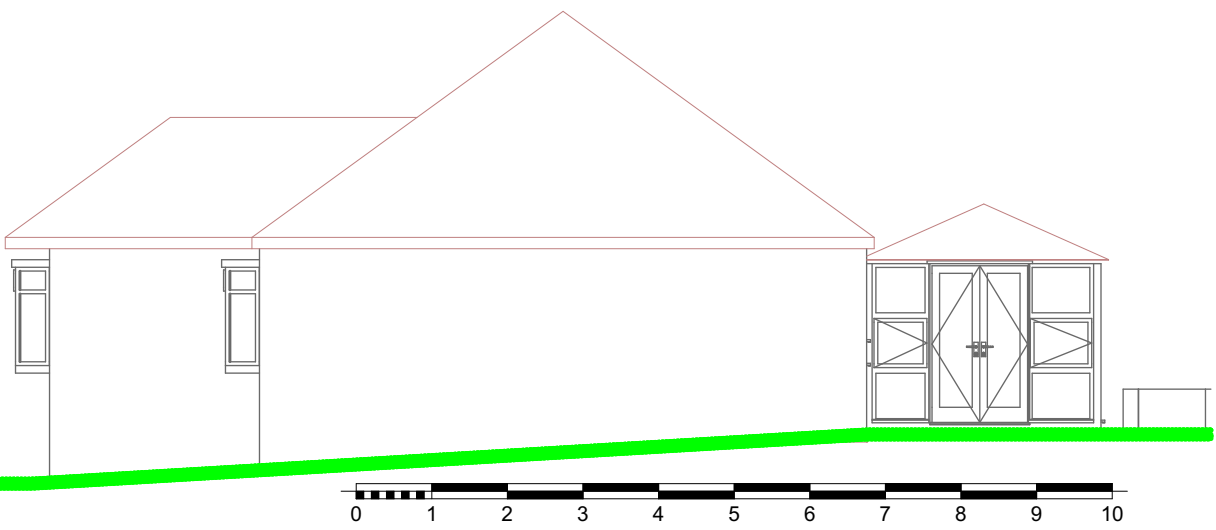
4 South Elevation Existing 1:100
