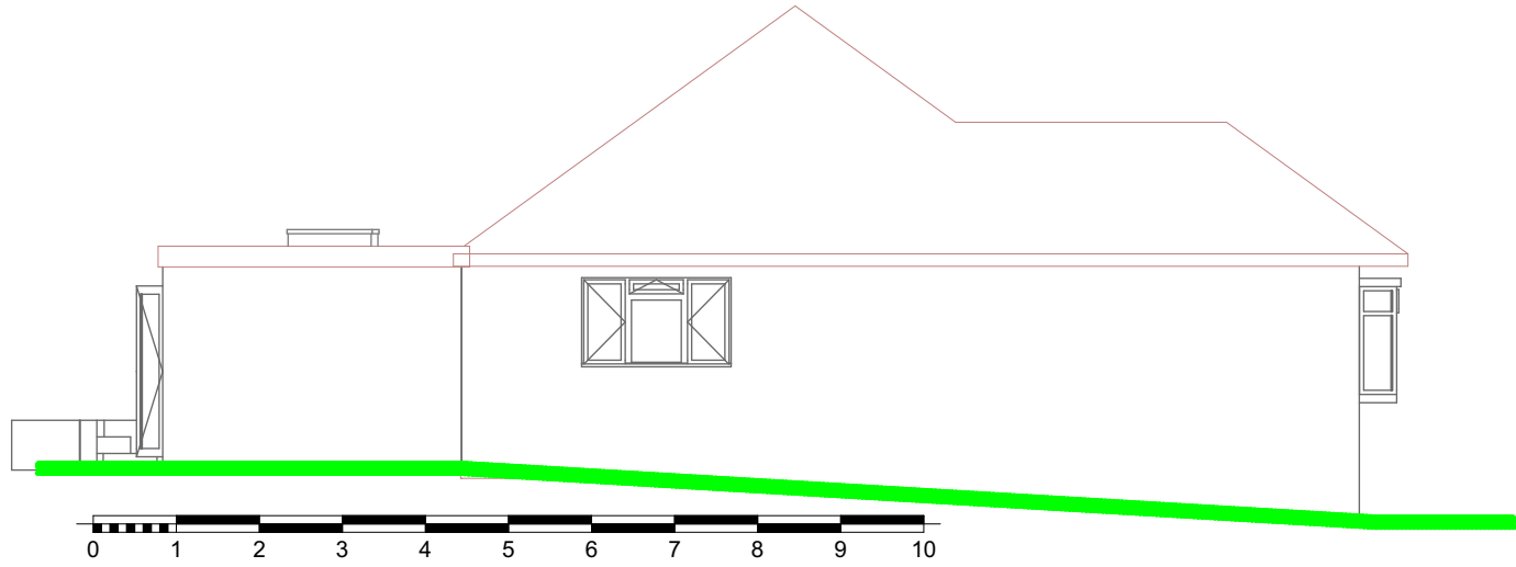
9 North Elevation Proposed 1:100
