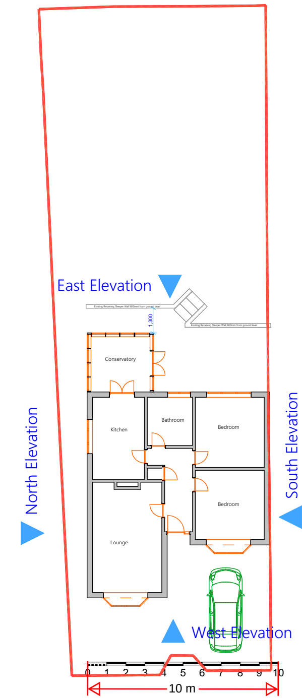
2 Site Plan Existing 1:200
