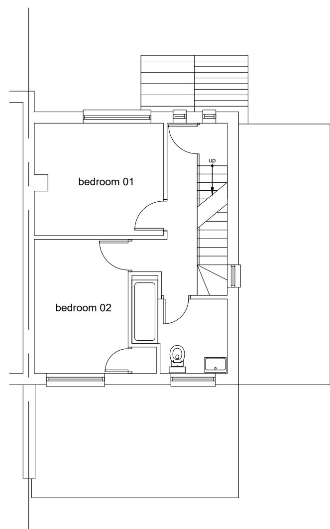
02 Existing First Floor Plan
