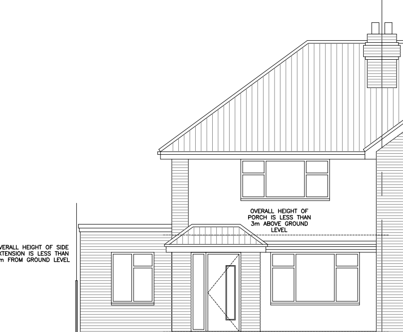
12 Proposed Front Elevation
