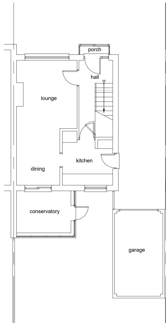
01 Existing Ground Floor Plan
