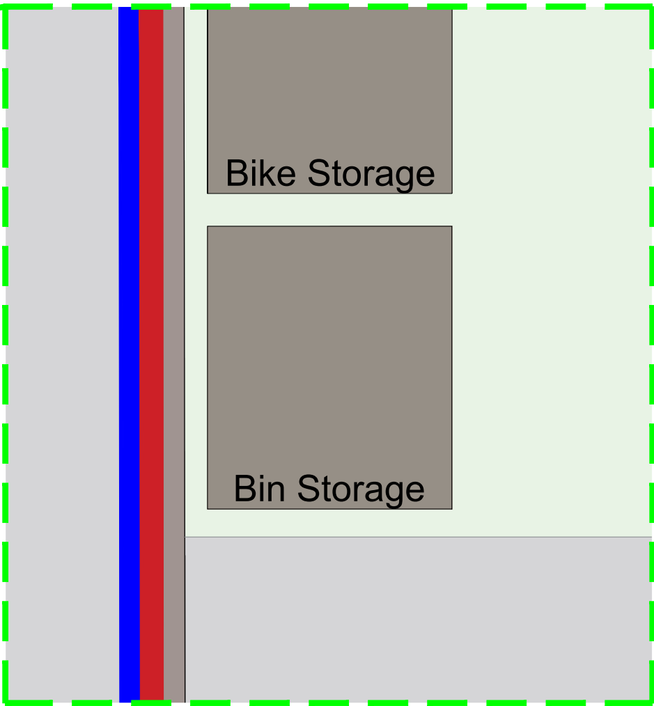
Refuse Storage 1:20
