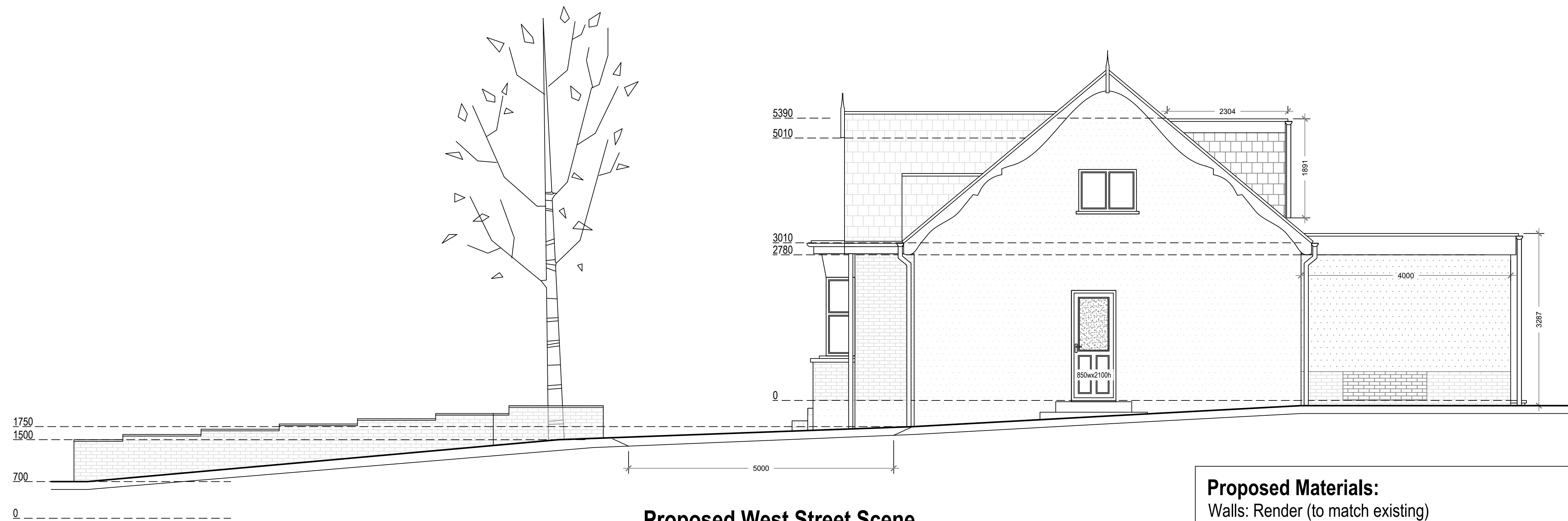
Proposed West Street Scene
