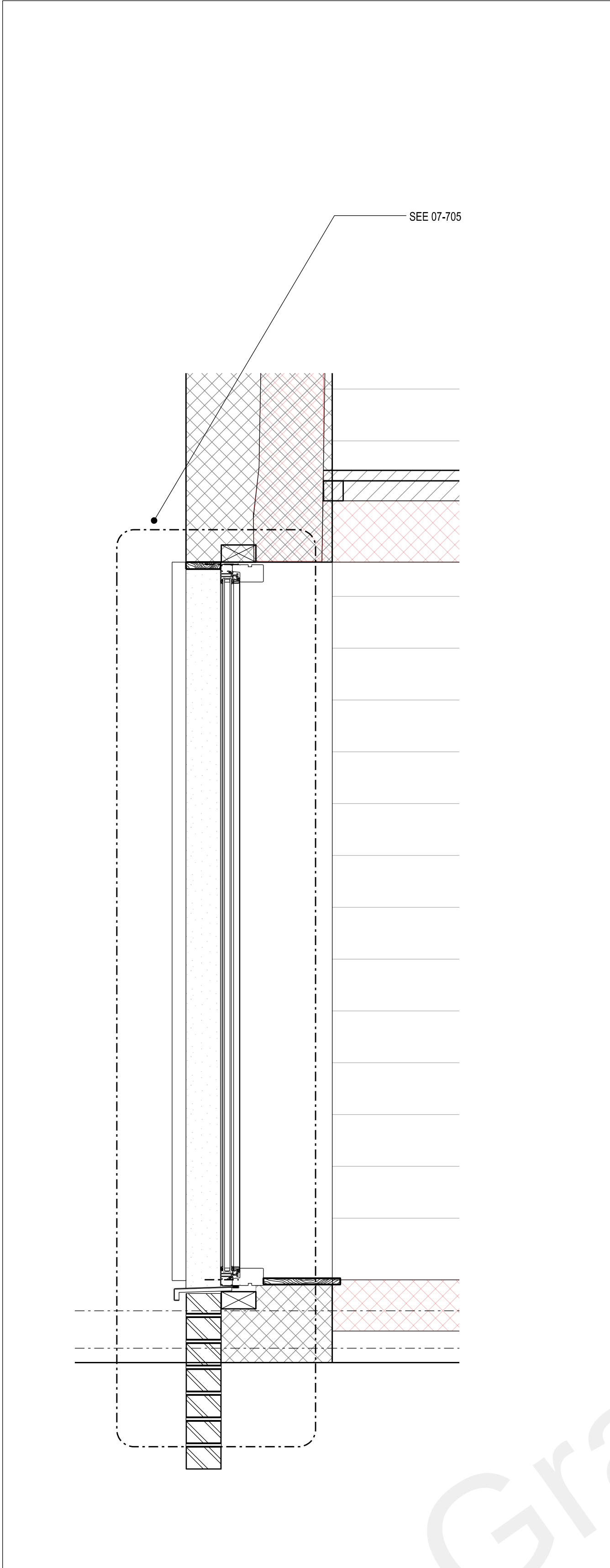
01 SECTION DETAIL
