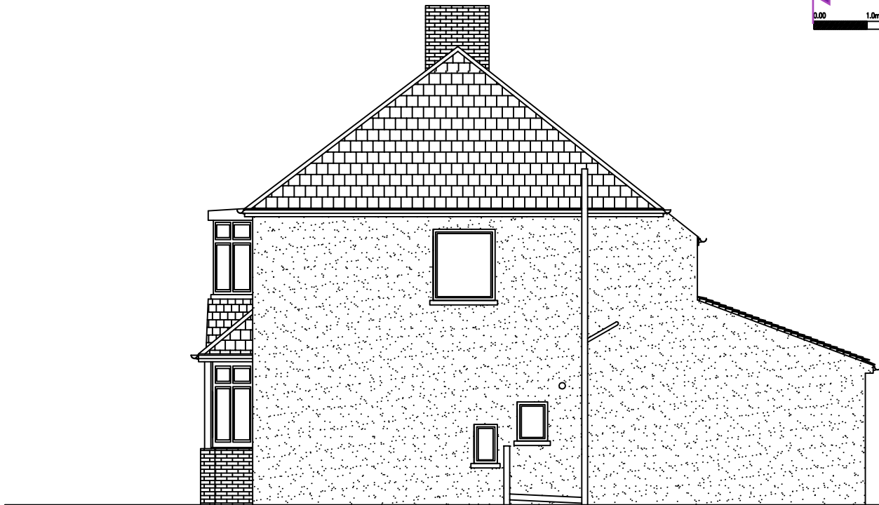
SIDE ELEVATION
