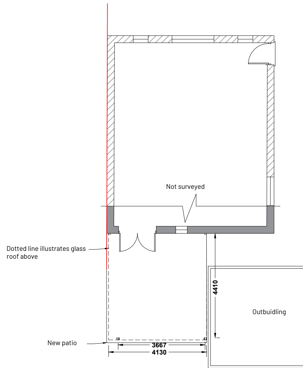
FLOOR PLAN
