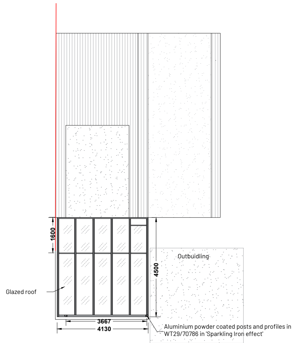
ROOF PLAN
