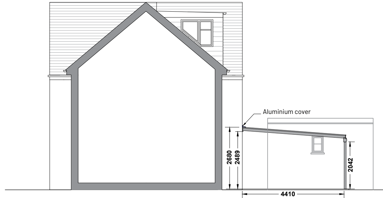
SIDE ELEVATION
