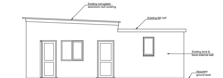
WEST ELEVATION
