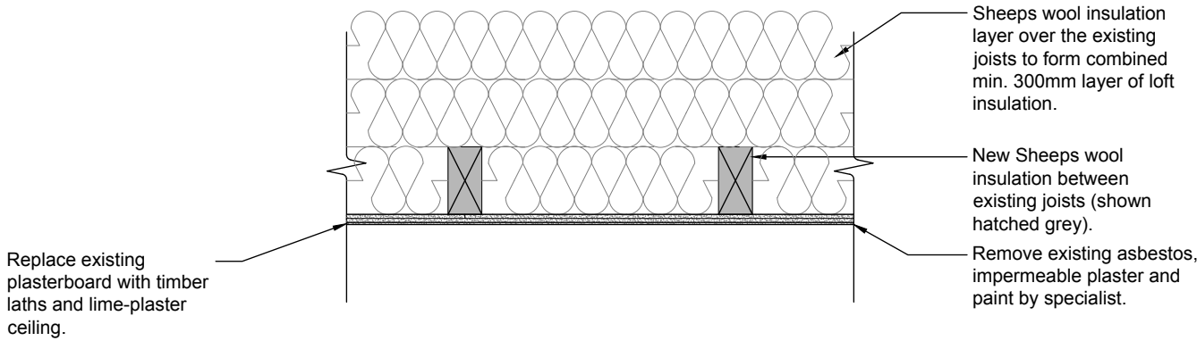
Proposed treatment to Ceiling Type 2 - Joist Line
