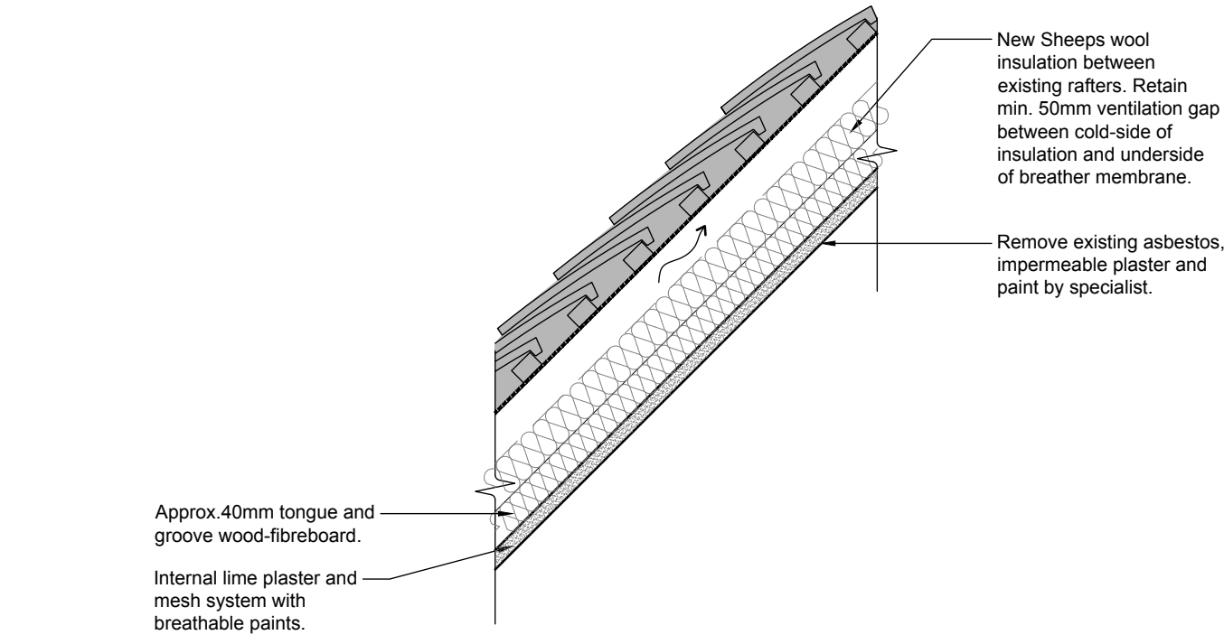
Proposed treatment to Ceiling Type 1 - Rafter Line
