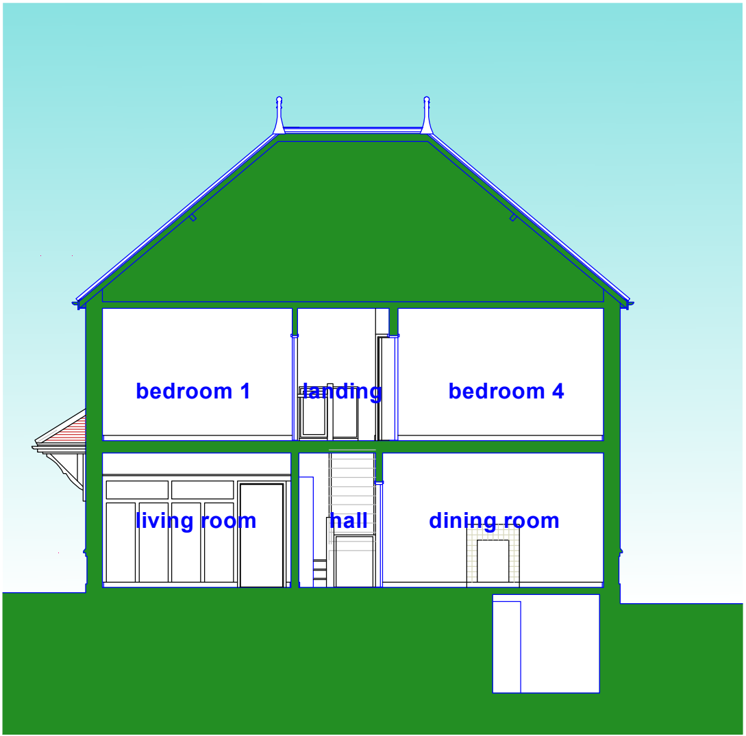
section bb
