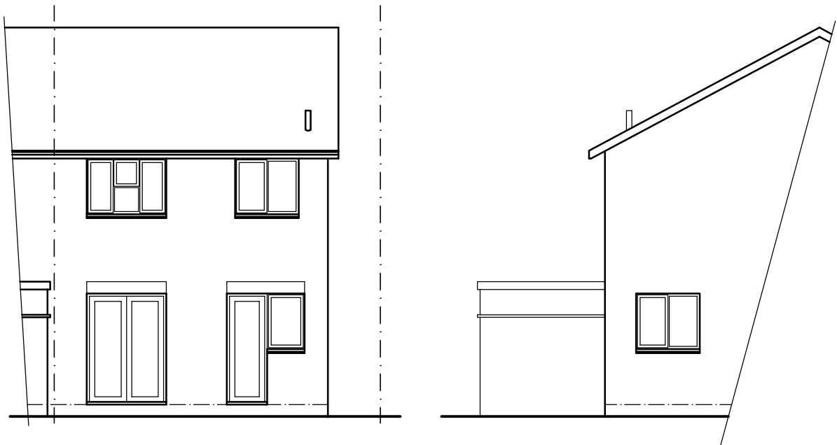
REAR ELEVATION (1:100)
