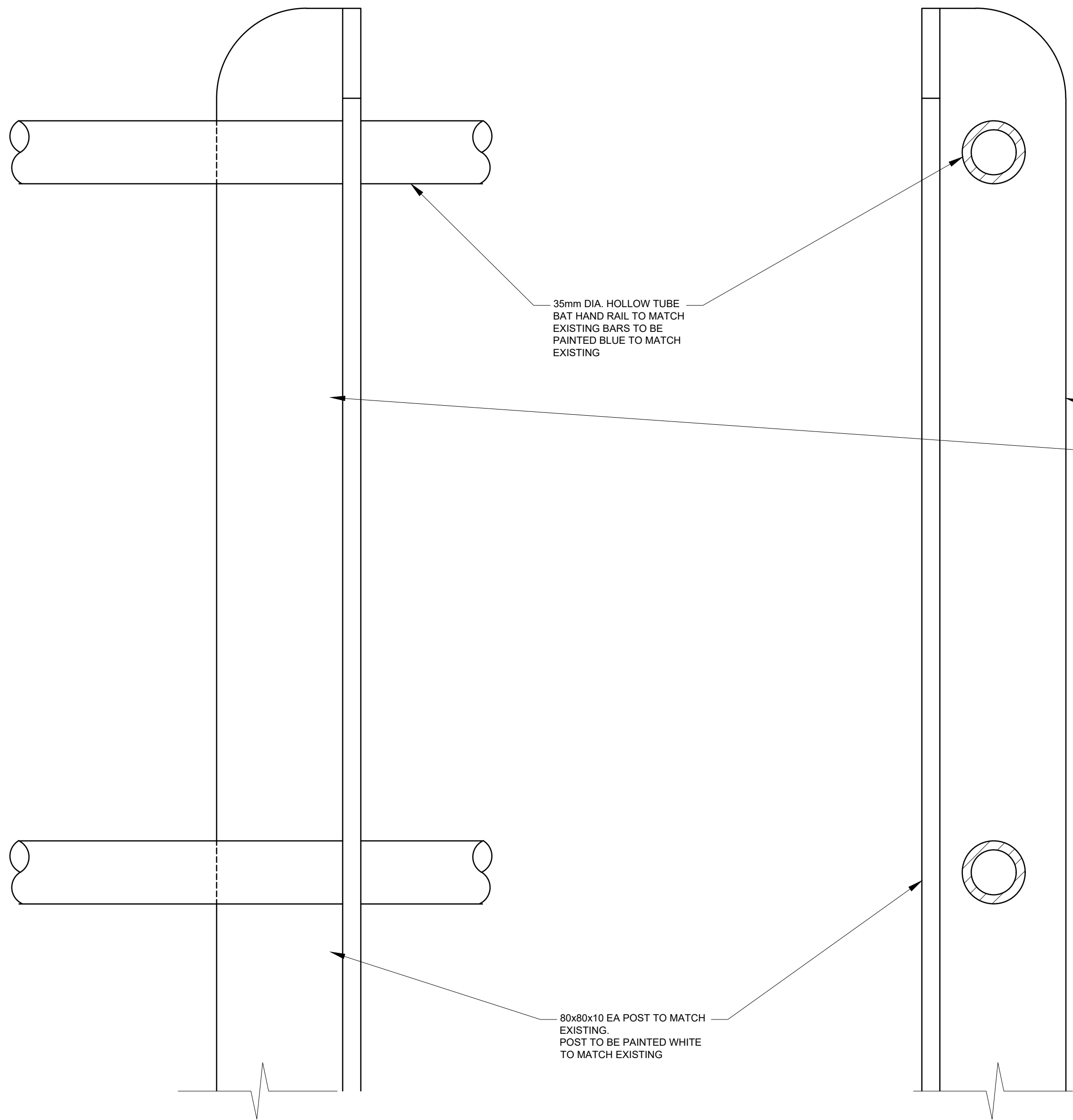
DETAIL 2 (ELEVATION)
