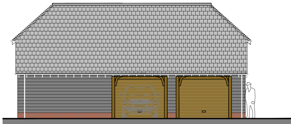
North Elevation (rear)
