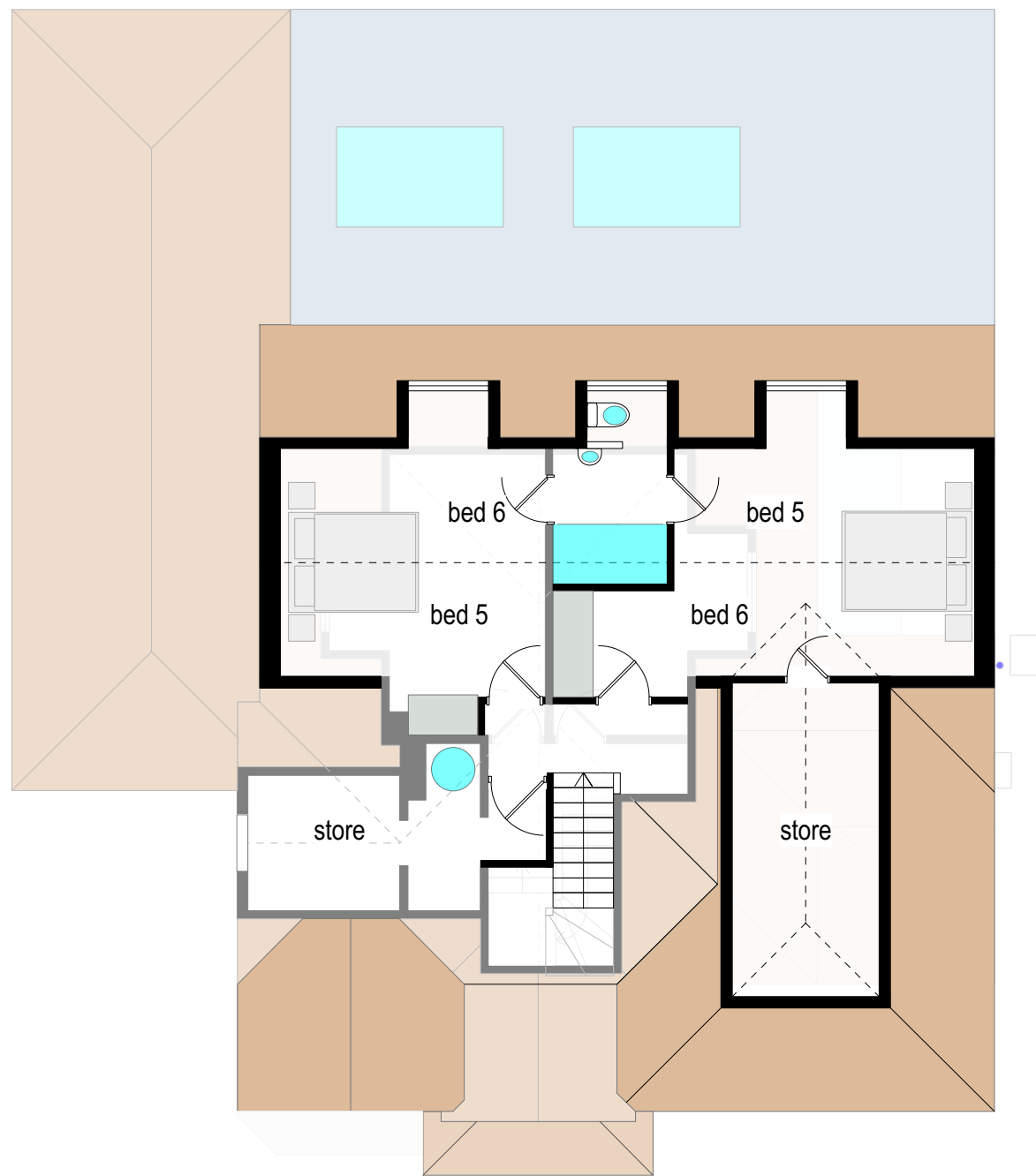
proposed attic floor plan - 60 sqm over 1.5m headroom
