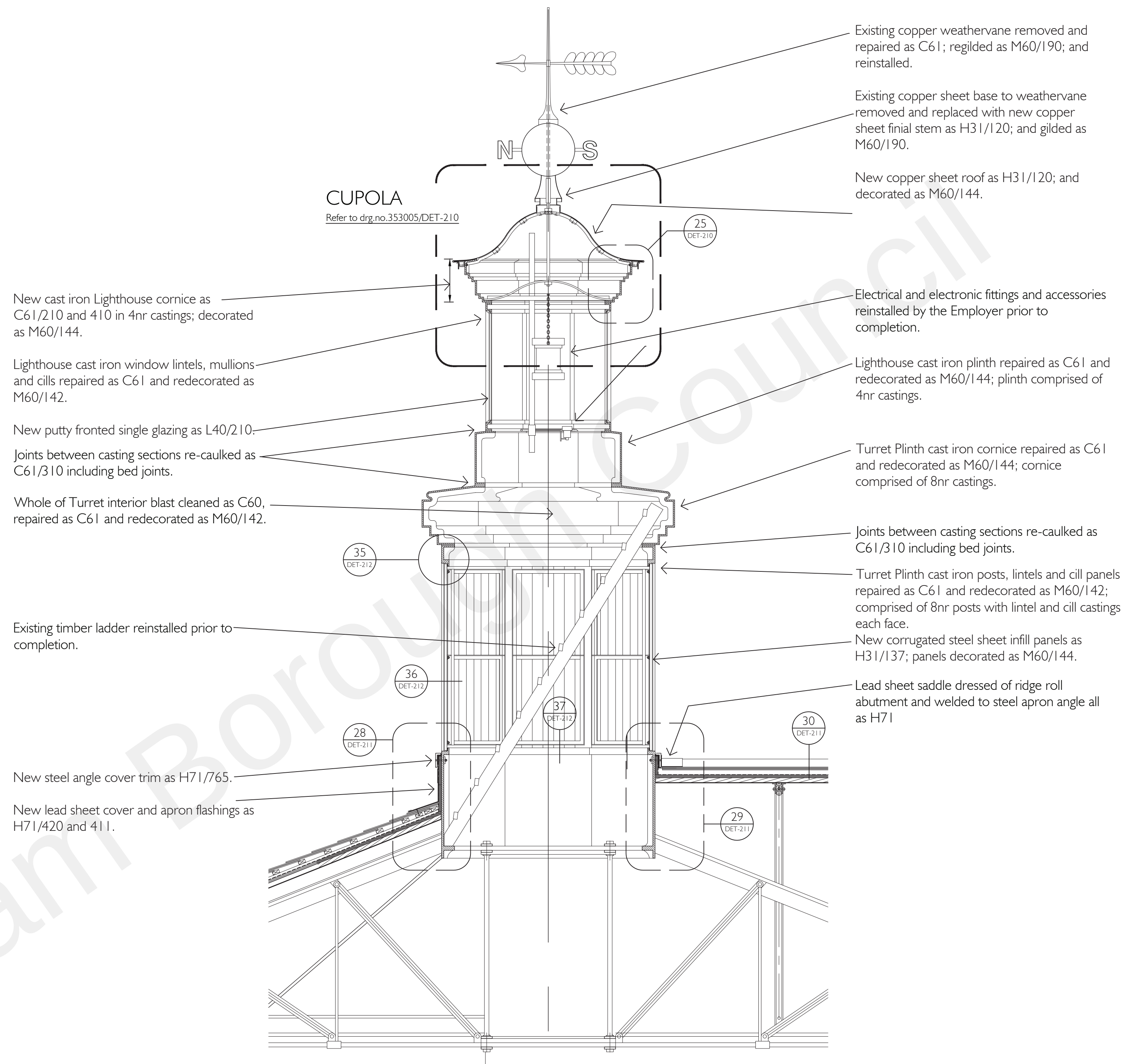
A - PIER HEAD LIGHT TURRET - SECTION A-A PROPOSED
