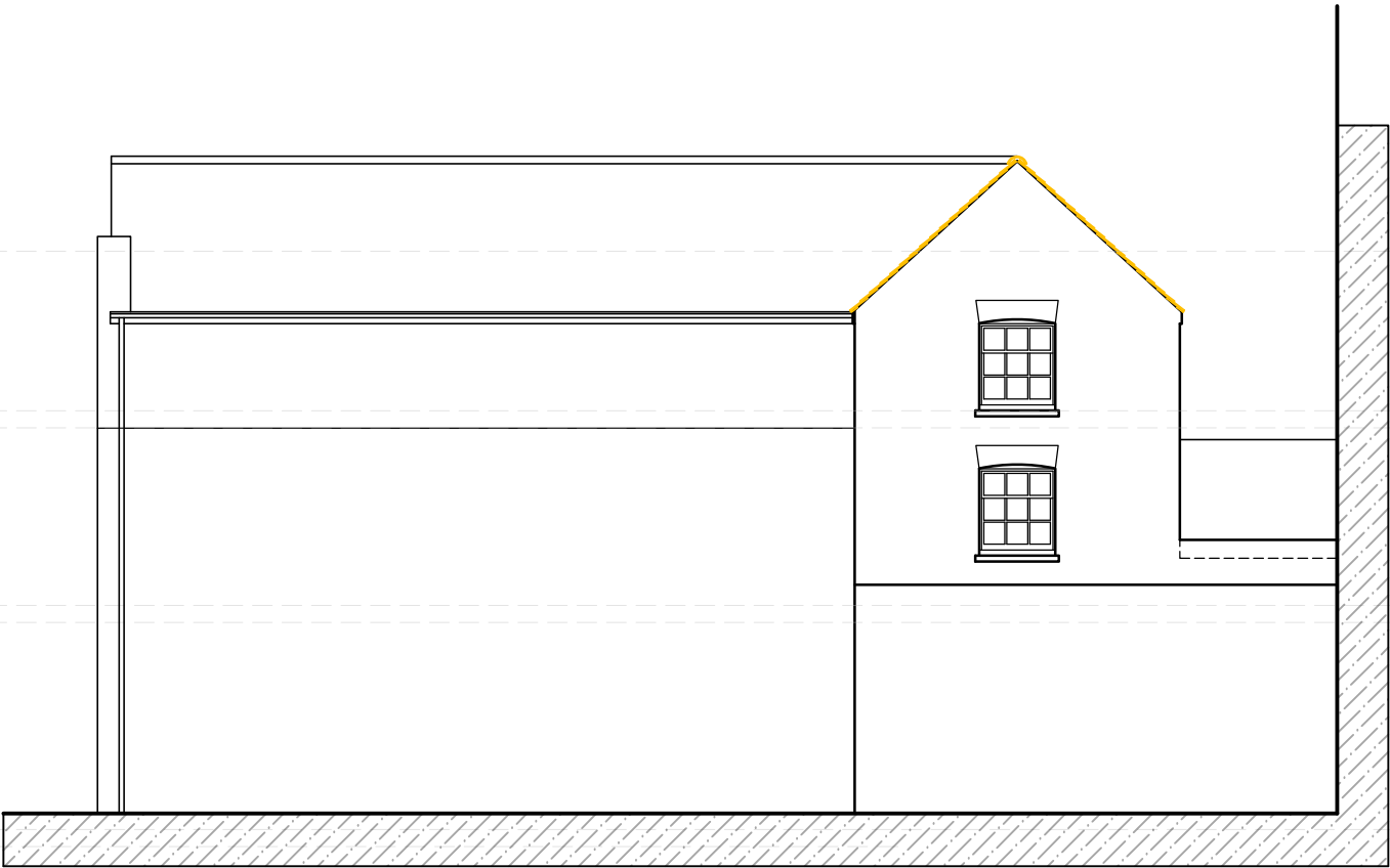
REAR ELEVATION (1:100)
