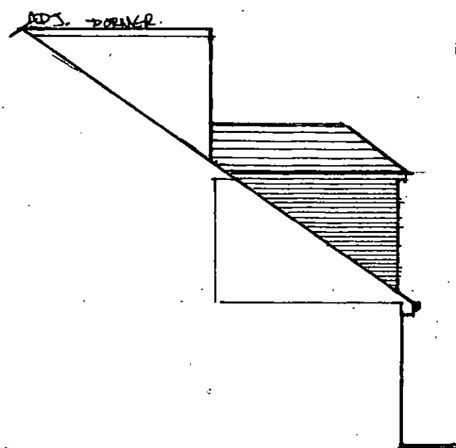
EXISTING SIDE ELEVATION AND PROPOSED SIDE ELEVATION
