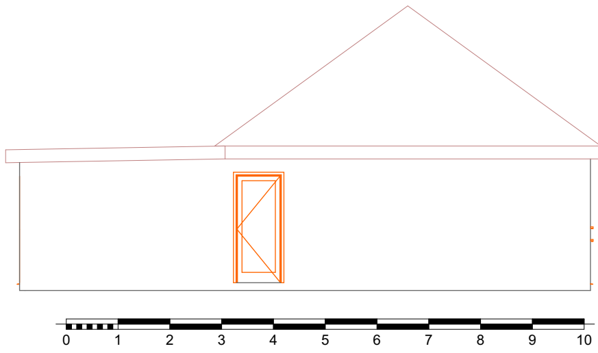
7 East Elevation Proposed 1:100
