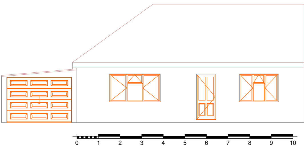
3 North Elevation Existing 1:100
