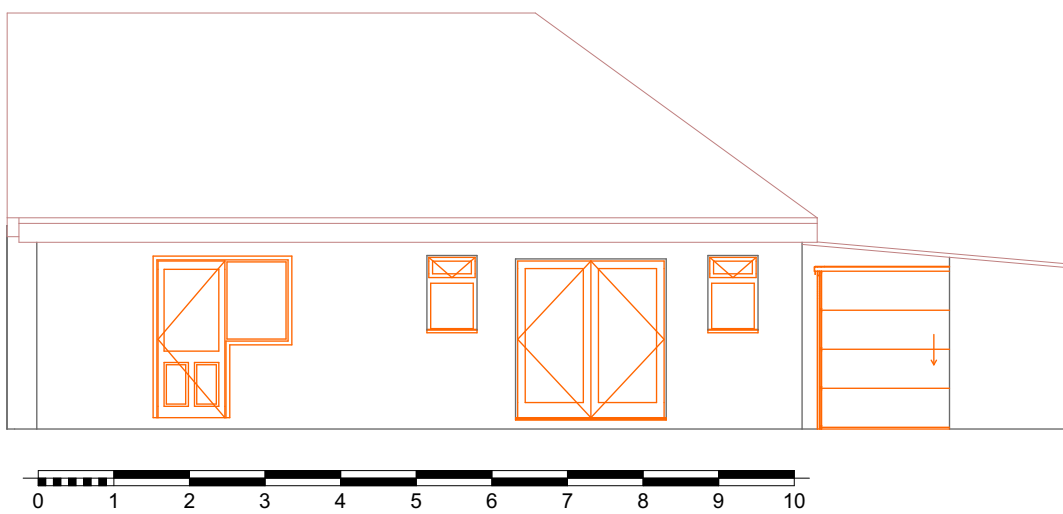
4 South Elevation Existing 1:100
