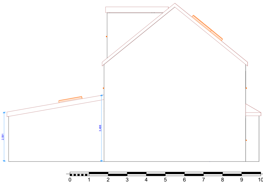
6 West Elevation Proposed 1:100
