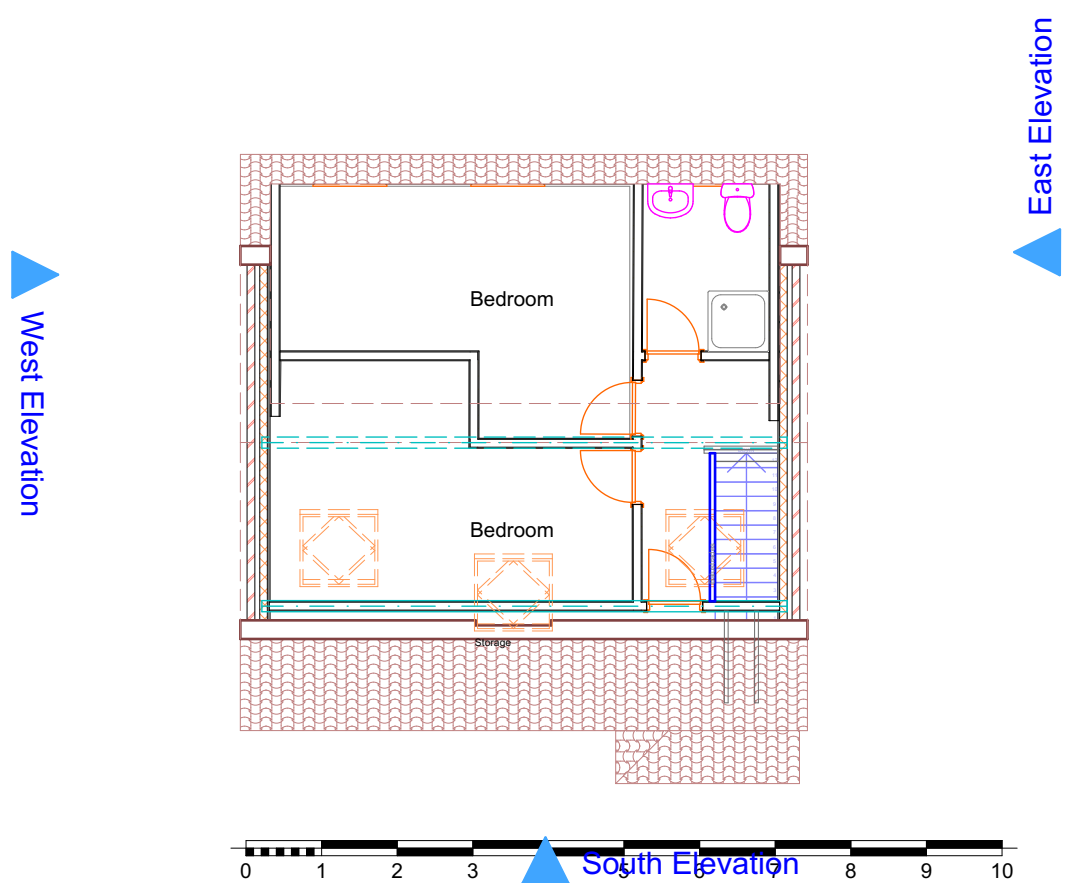
3 Roof-Existing 1:100
