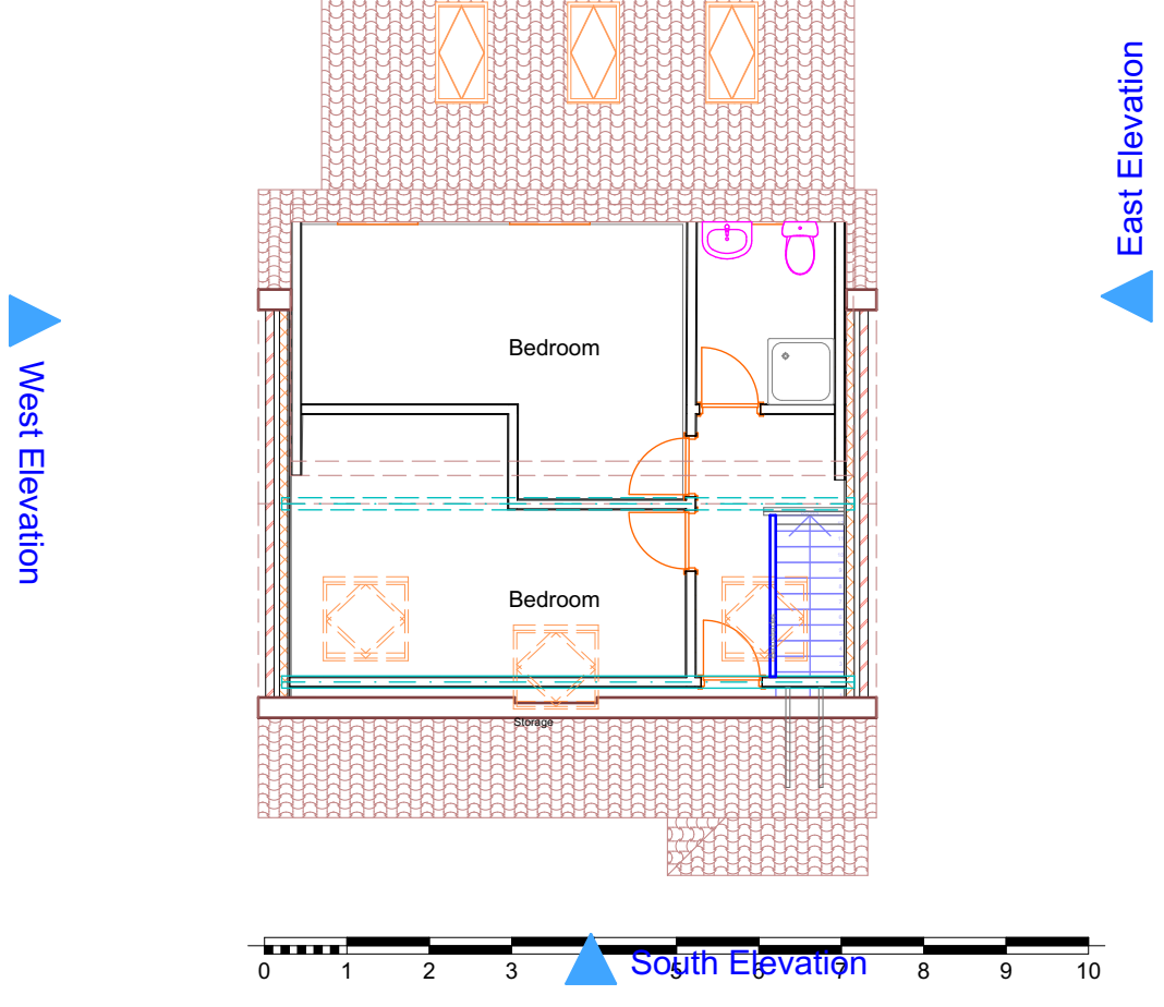
6 Roof Proposed 1:100
