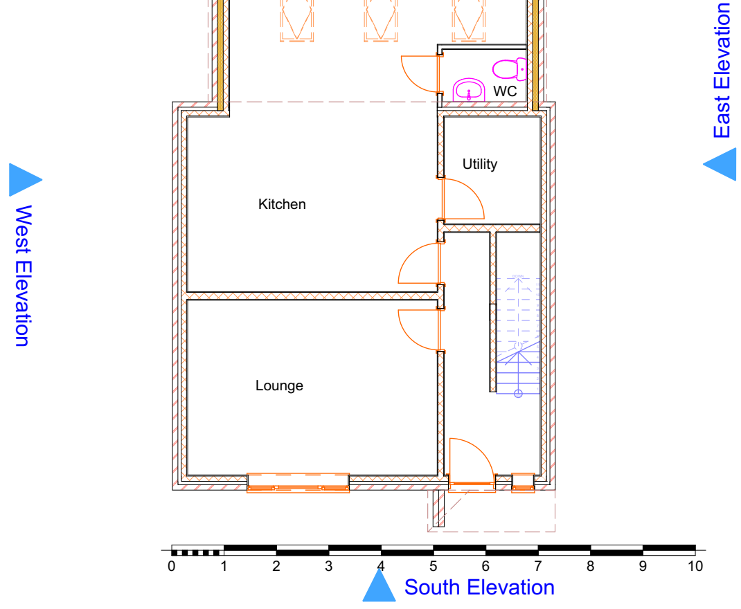
4 GF Ground Floor Proposed 1:100
