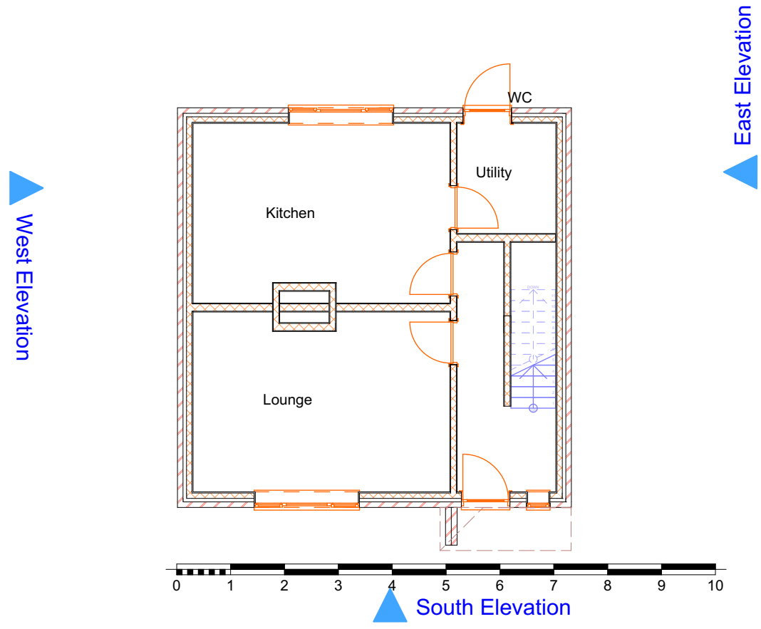
1 GF Ground Floor Existing 1:100
