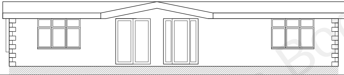
Existing West Elevation 1:100
