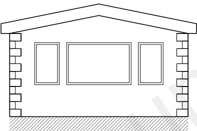
Existing North Elevation 1:100
