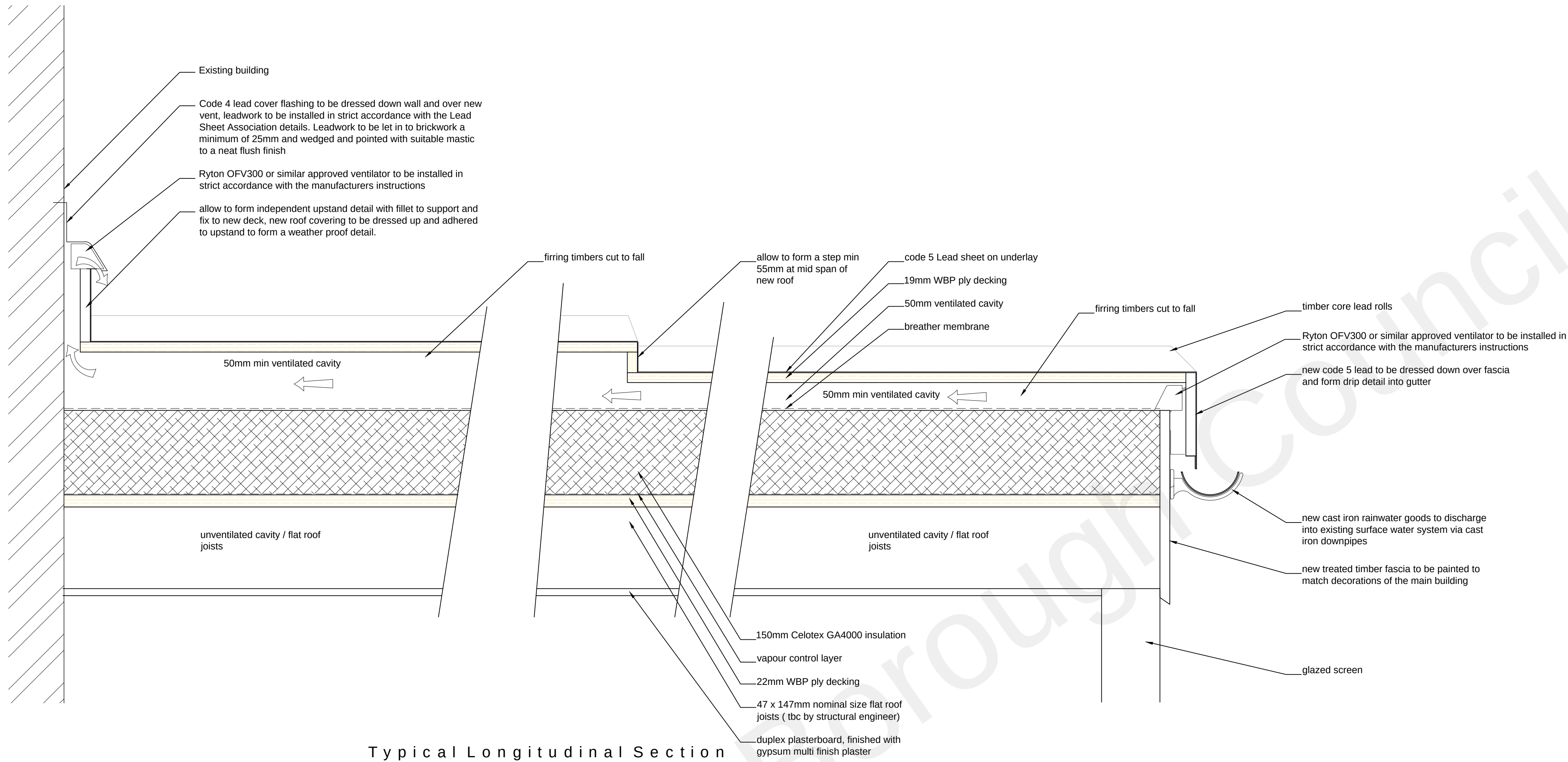
Typical Longitudinal Section
