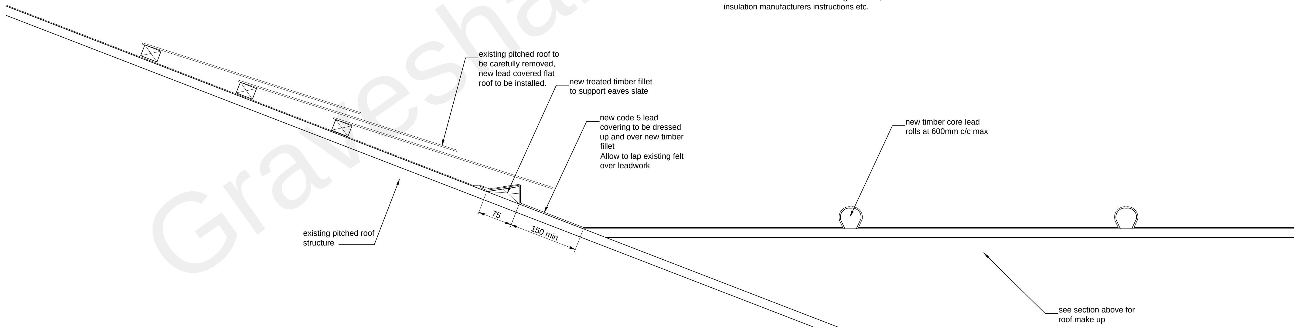
Typical Section at junction with Existing Pitched Roof
