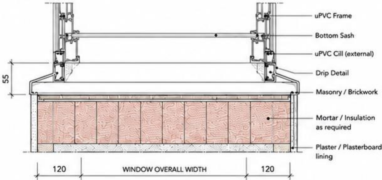
03 CILL SECTION SCALE 1:10
