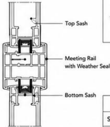
04 MEETING RAIL DETAIL SCALE 1:10
