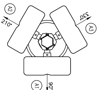
PROPOSED ANTENNA PLAN (UPPER)
