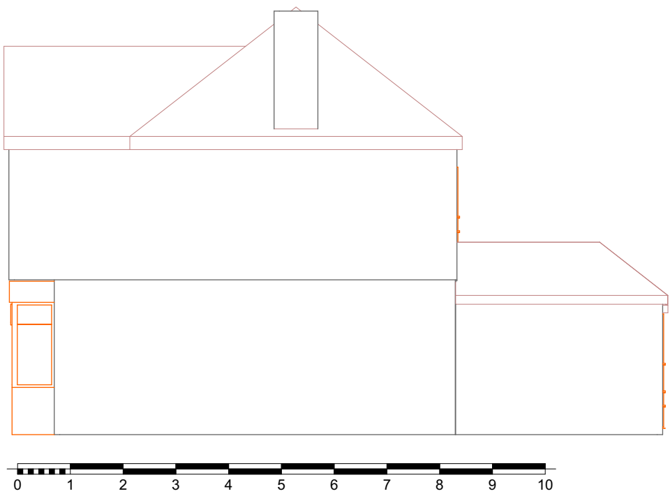
1 East Elevation Existing 1:100
