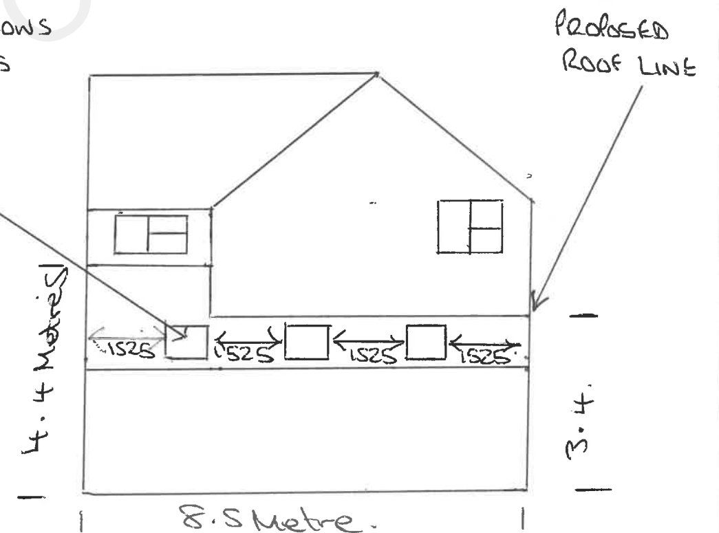
8.5 Metre. PROPOSED ELEVATION
