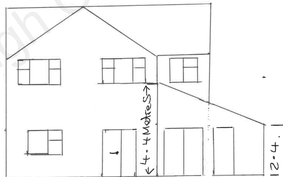
PROPOSED ELEVATION
