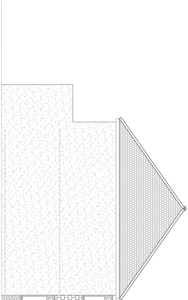
EXISTING NORTH WEST FACING SIDE ELEVATION
