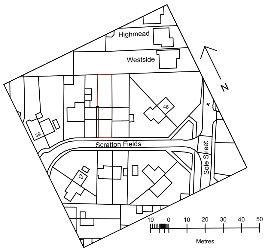
1 Location Plan 1:1250
