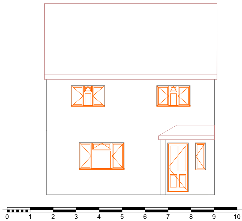
4 South Elevation Existing 1:100
