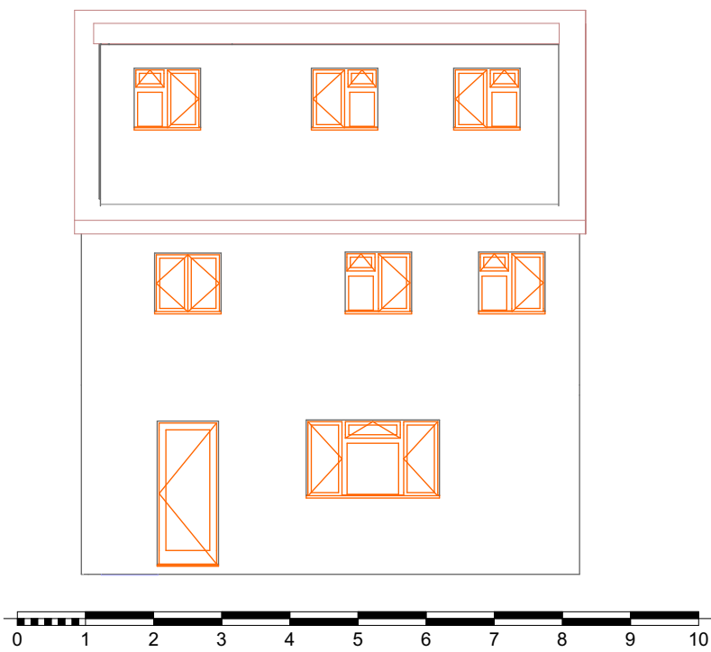
3 North Elevation Existing 1:100
