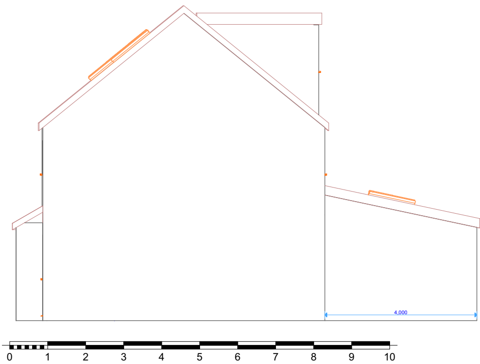
5 East Elevation Proposed 1:100
