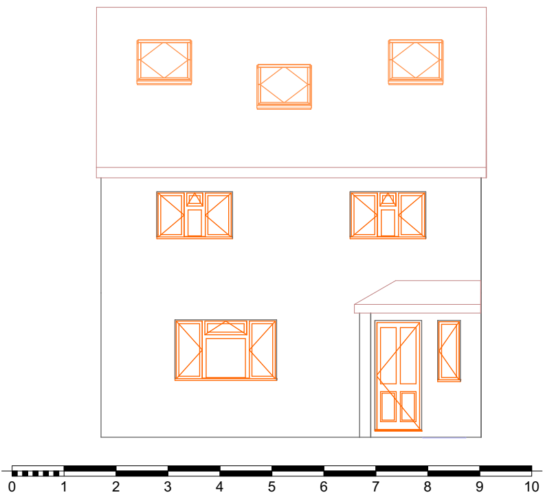
8 South Elevation Proposed 1:100
