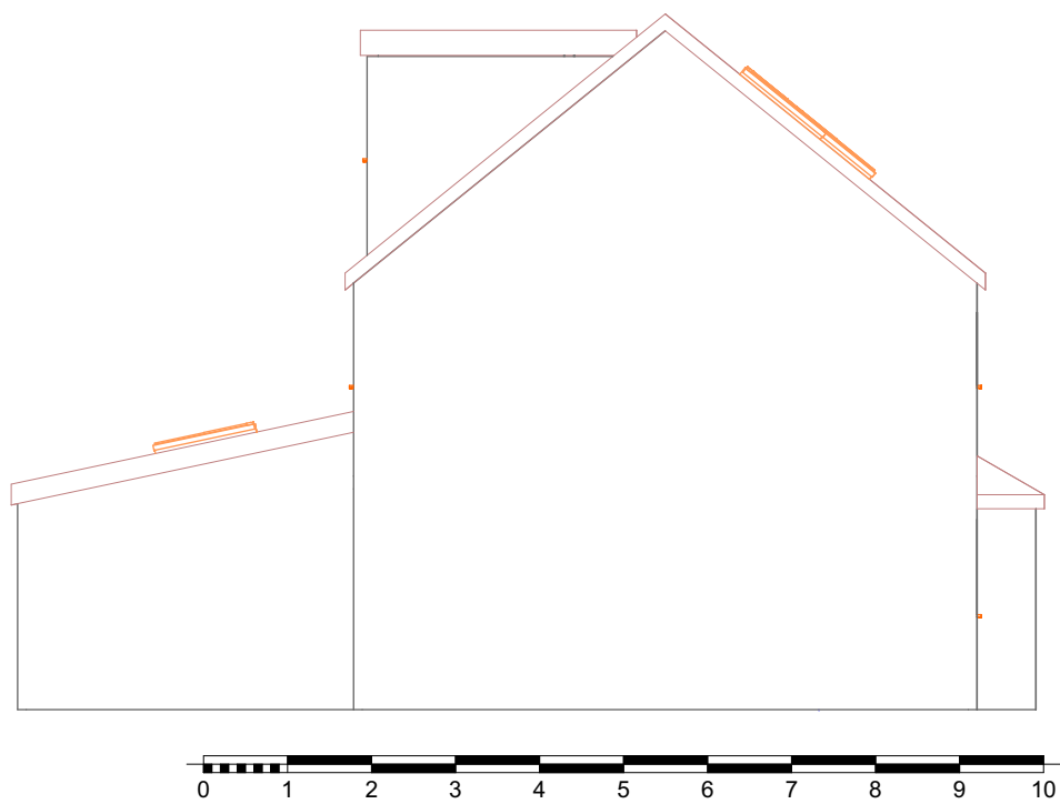
6 West Elevation Proposed 1:100
