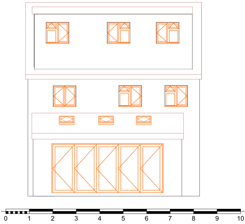
6 West Elevation Proposed 1:100
