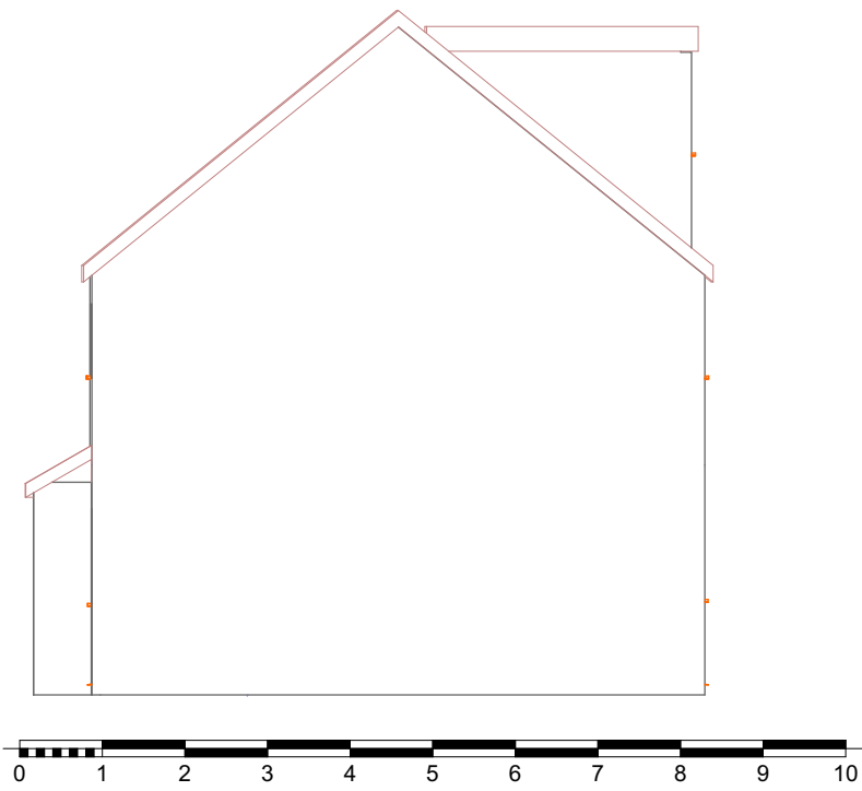
1 East Elevation Existing 1:100
