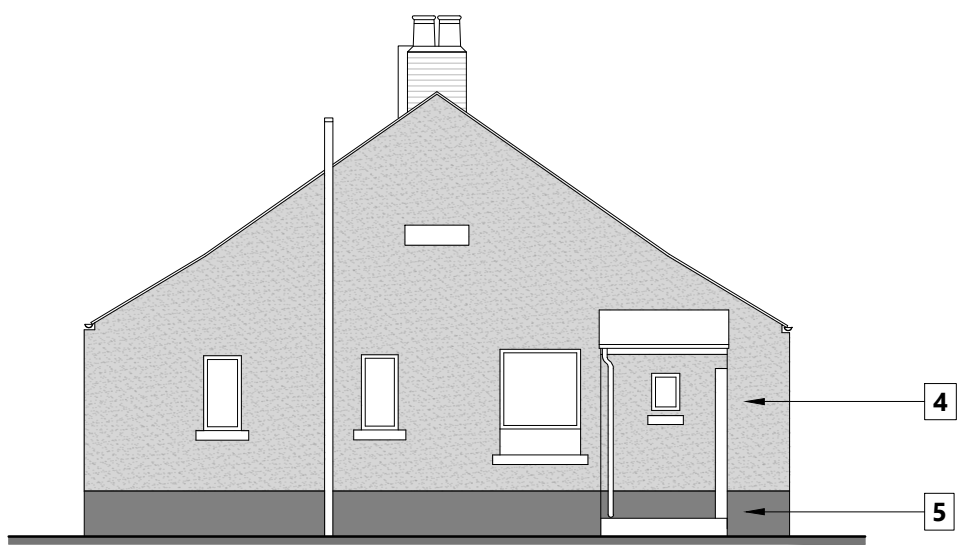
East Elevation
