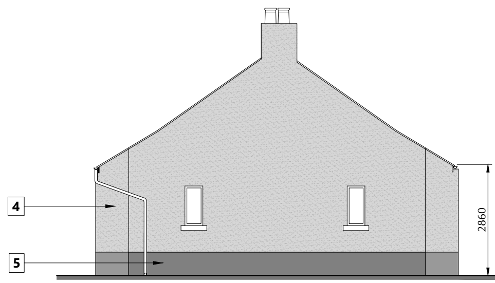
West Elevation
