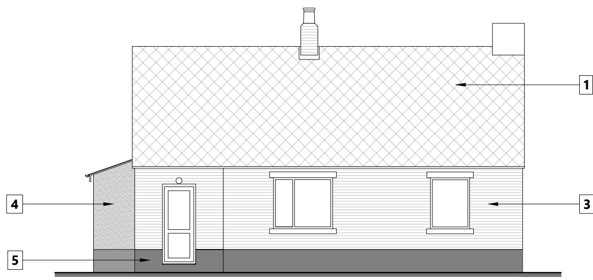
North Elevation
