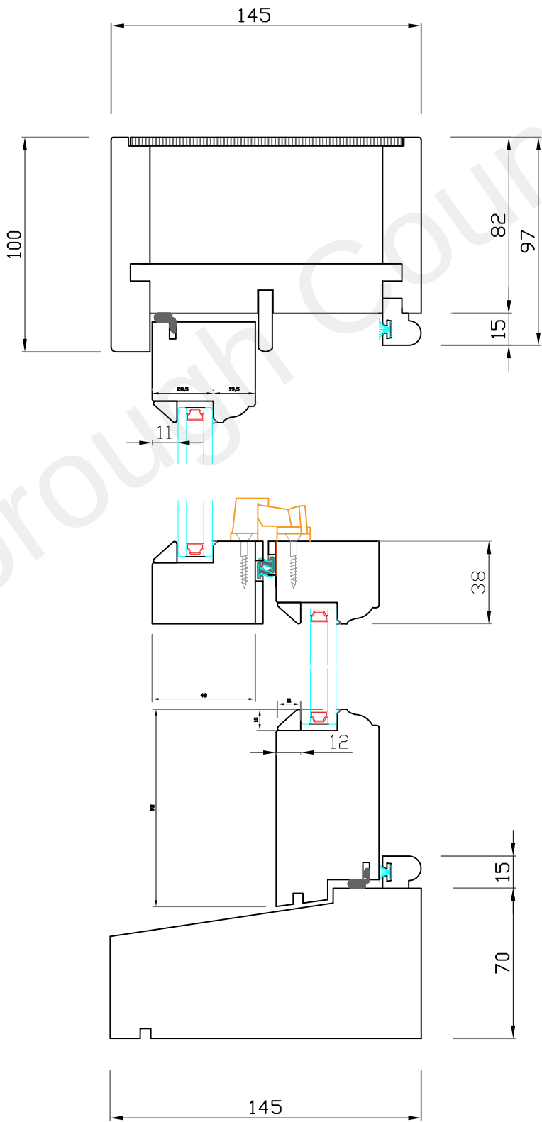
Horizontal section
