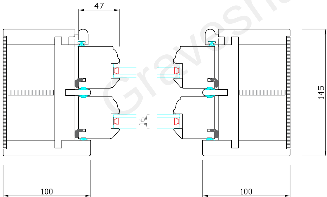
Vertical sections
