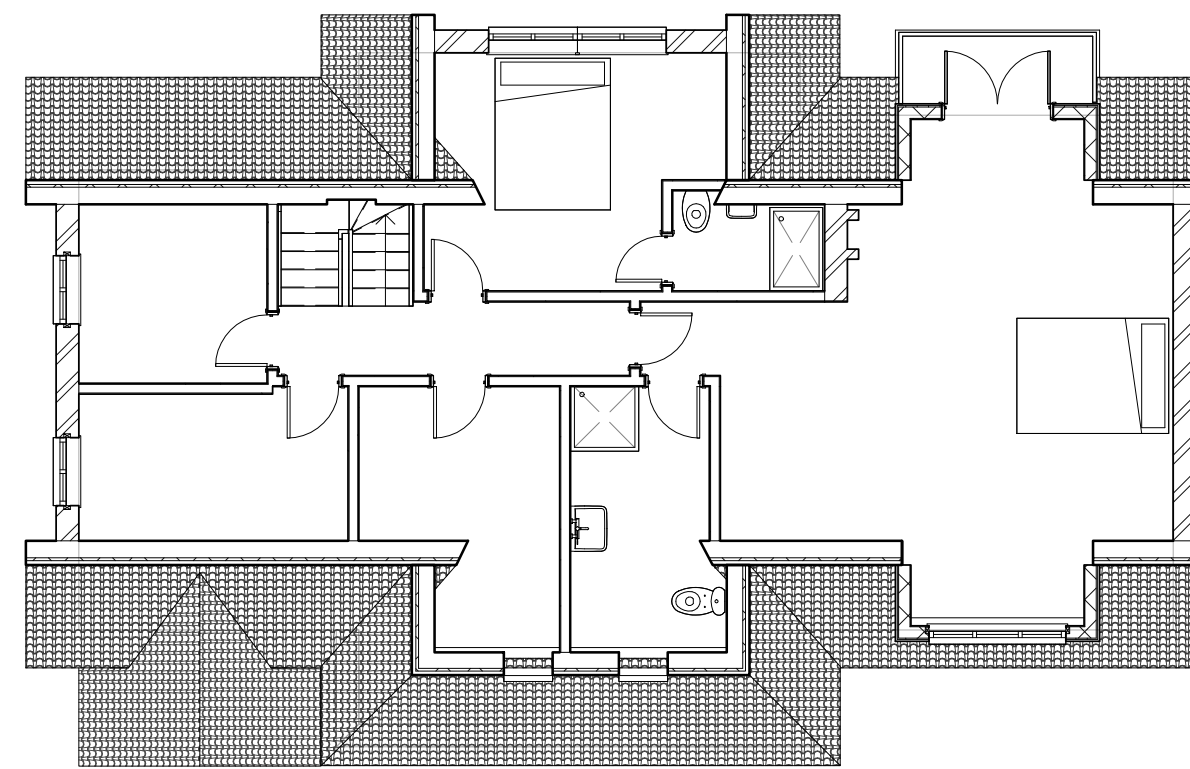
2 FIRST FLOOR 1 : 100
