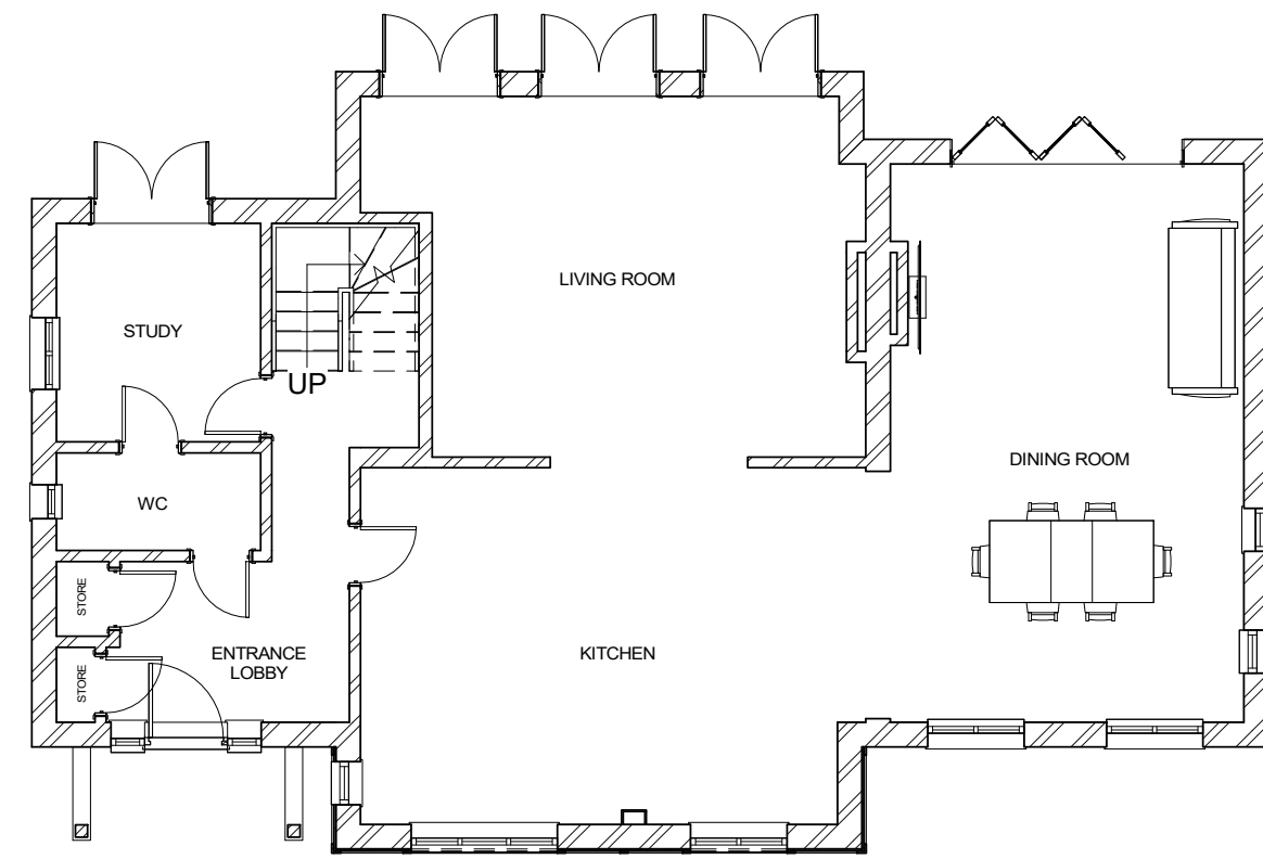
1 GROUND FLOOR 1 : 100
