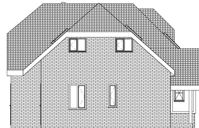
4 NORTHSIDE ELEVATION 1 : 100
