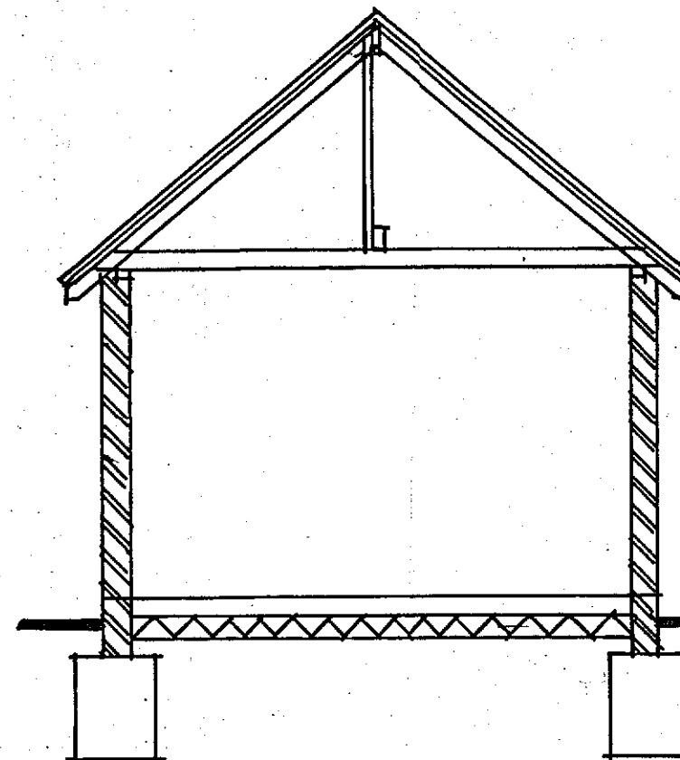
CROSS SECTION
