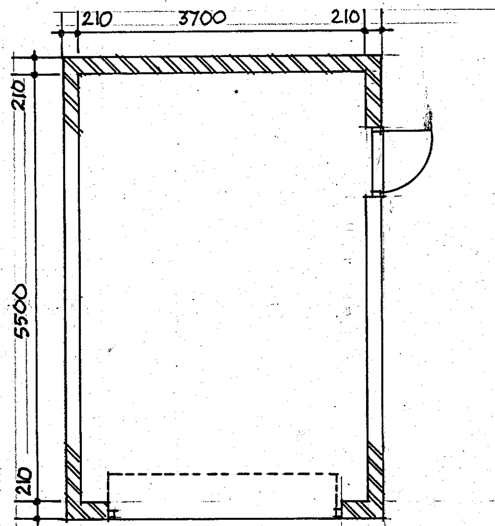
PLAN
