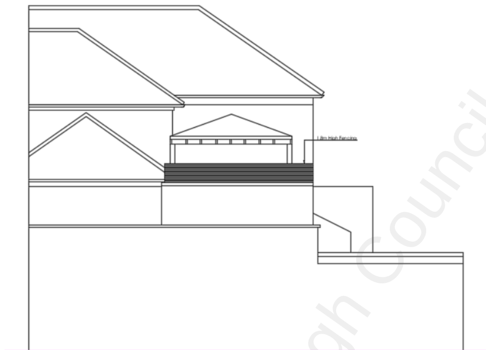
REAR ELEVATION
