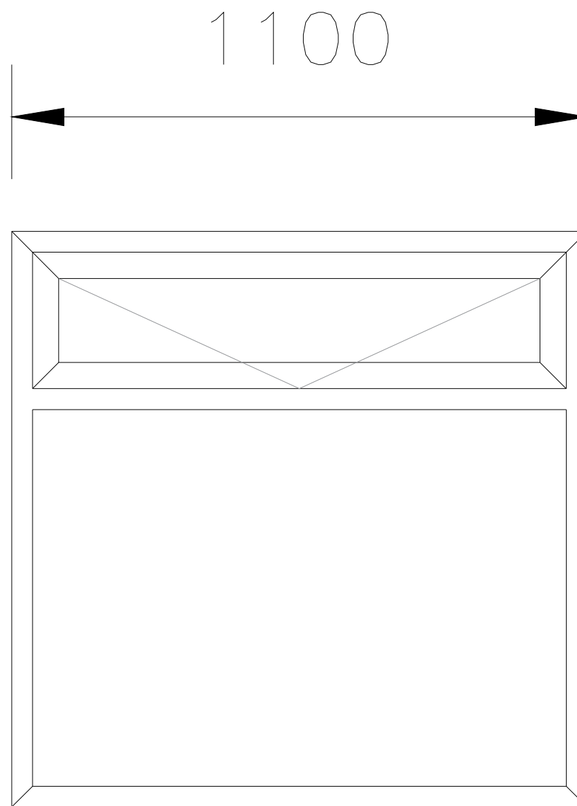
External Elevation 1:10
