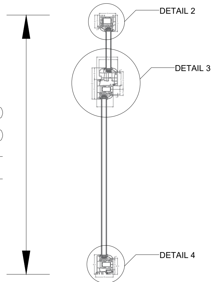
Vertical Cross-section 1:10
