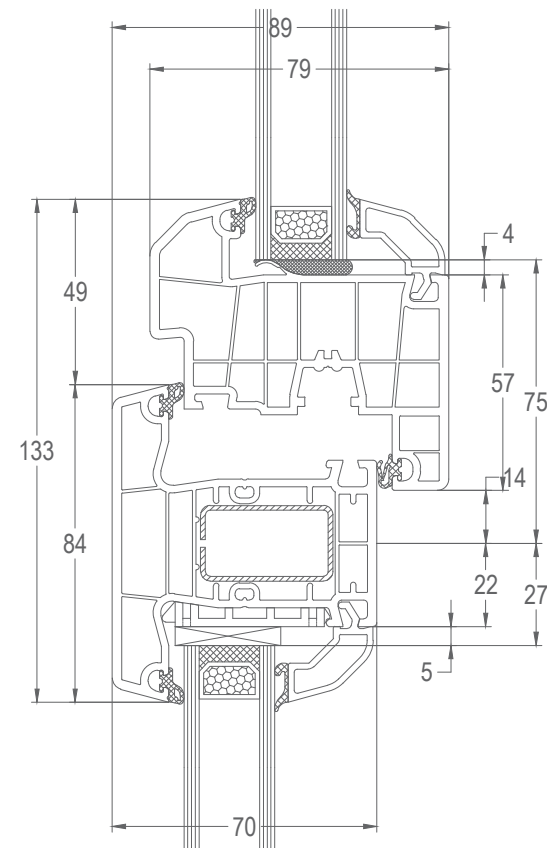
DETAIL 3
