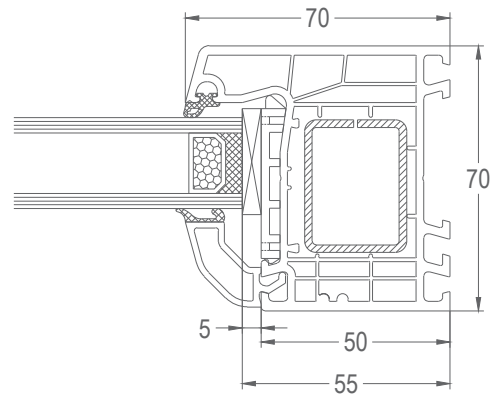
DETAIL 1
