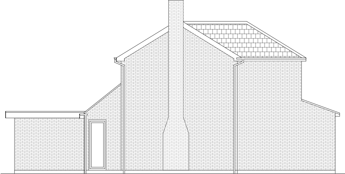
Proposed west
