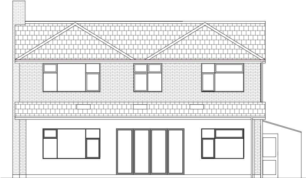
Proposed south
