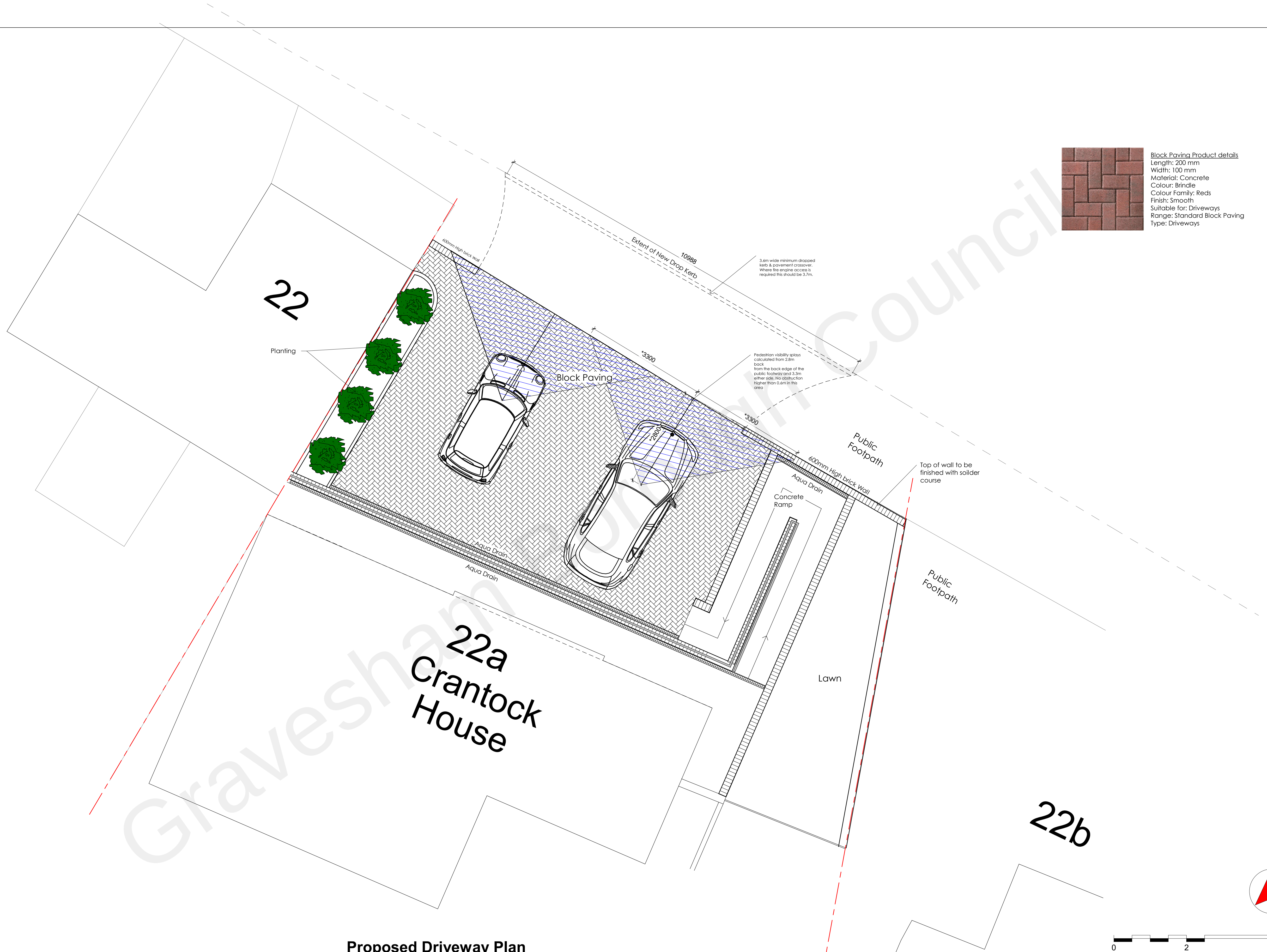
Proposed Driveway Plan 1 : 50
