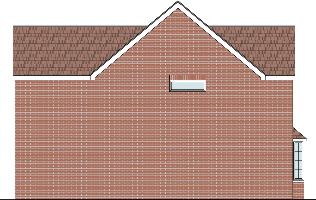
Proposed South-East Elevation (Side)
