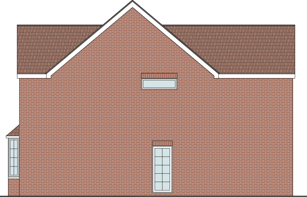
Proposed North-West Elevation (Side)
