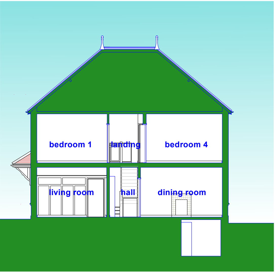
section bb
