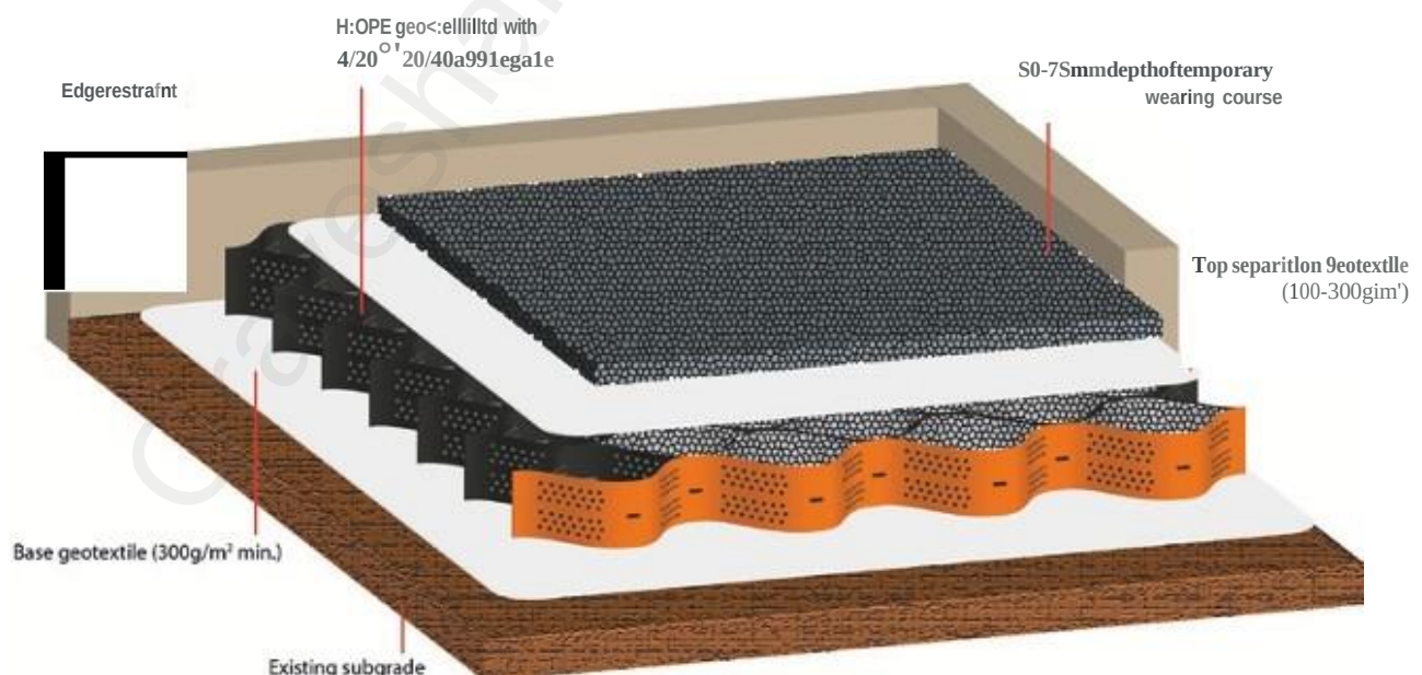
Figure 5: A geocell surface used during construction needs to be protected by a temporary wearing course and an upper geotextile is required to prevent mud from migrating down into the infill stone aggregate.
