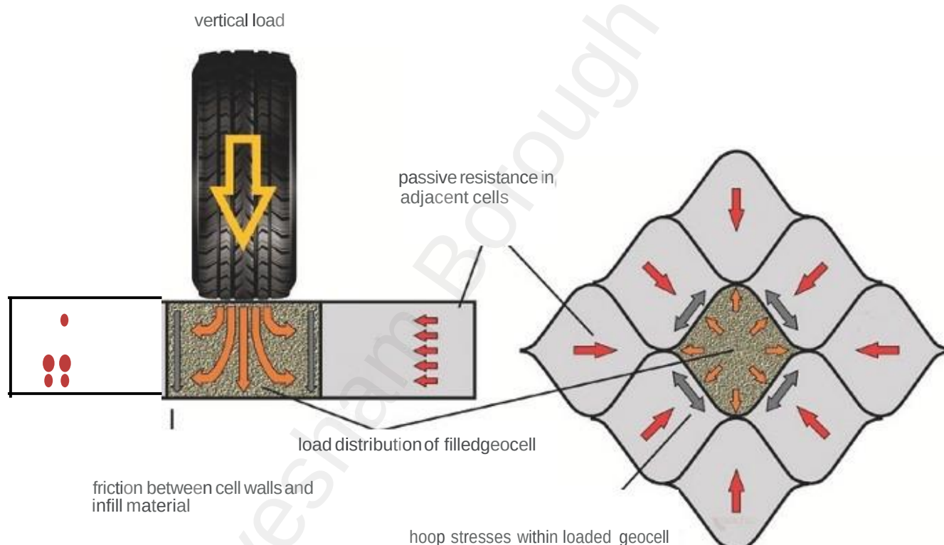
Figure 3: This diagram illustrates the forces and stress distribution when a vertical load is applied to a cellular confinement system (image courtesy of Professor Geosynesis [Greenix])
