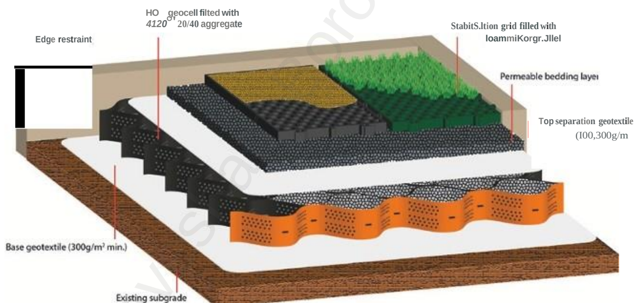
Figure 7: The sub-base configuration required for gravel or grass surfacing, from the core LPJ
