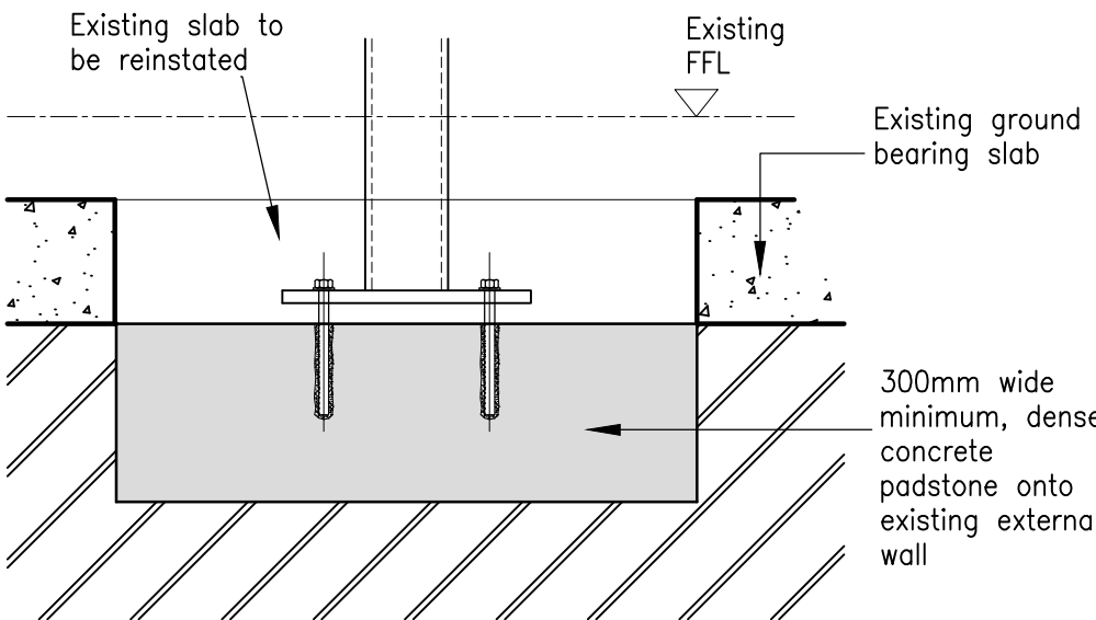
Typical Column Padstone Detail Scale at 1:10
