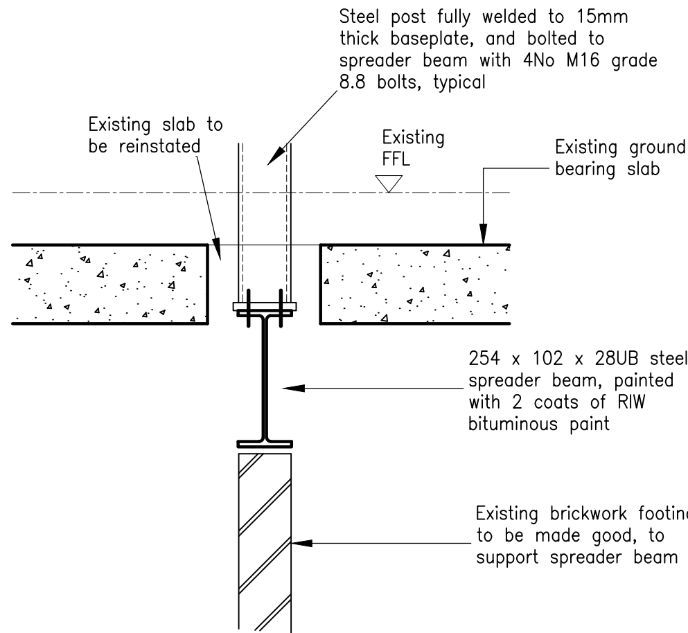
Section through Spreader Beam Scale at 1:10
