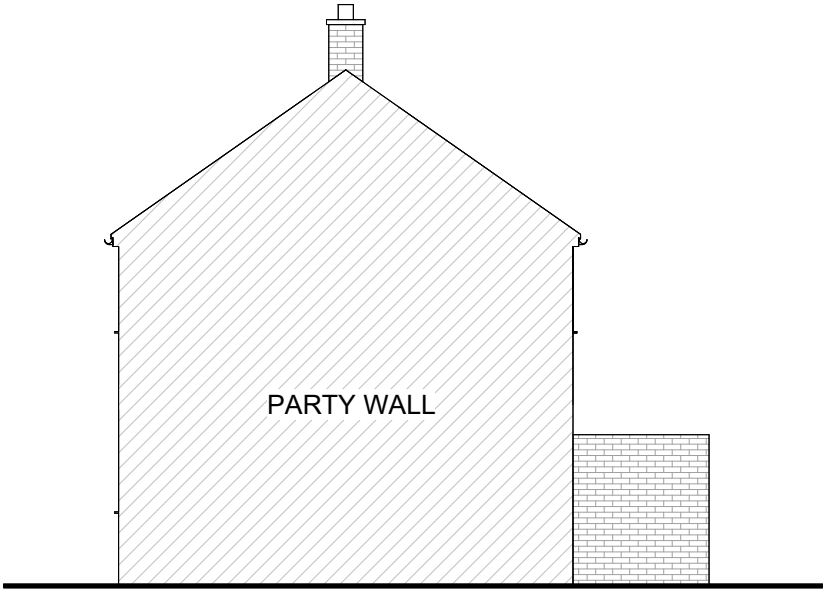
2 Side Elevation (South) 1 : 100
