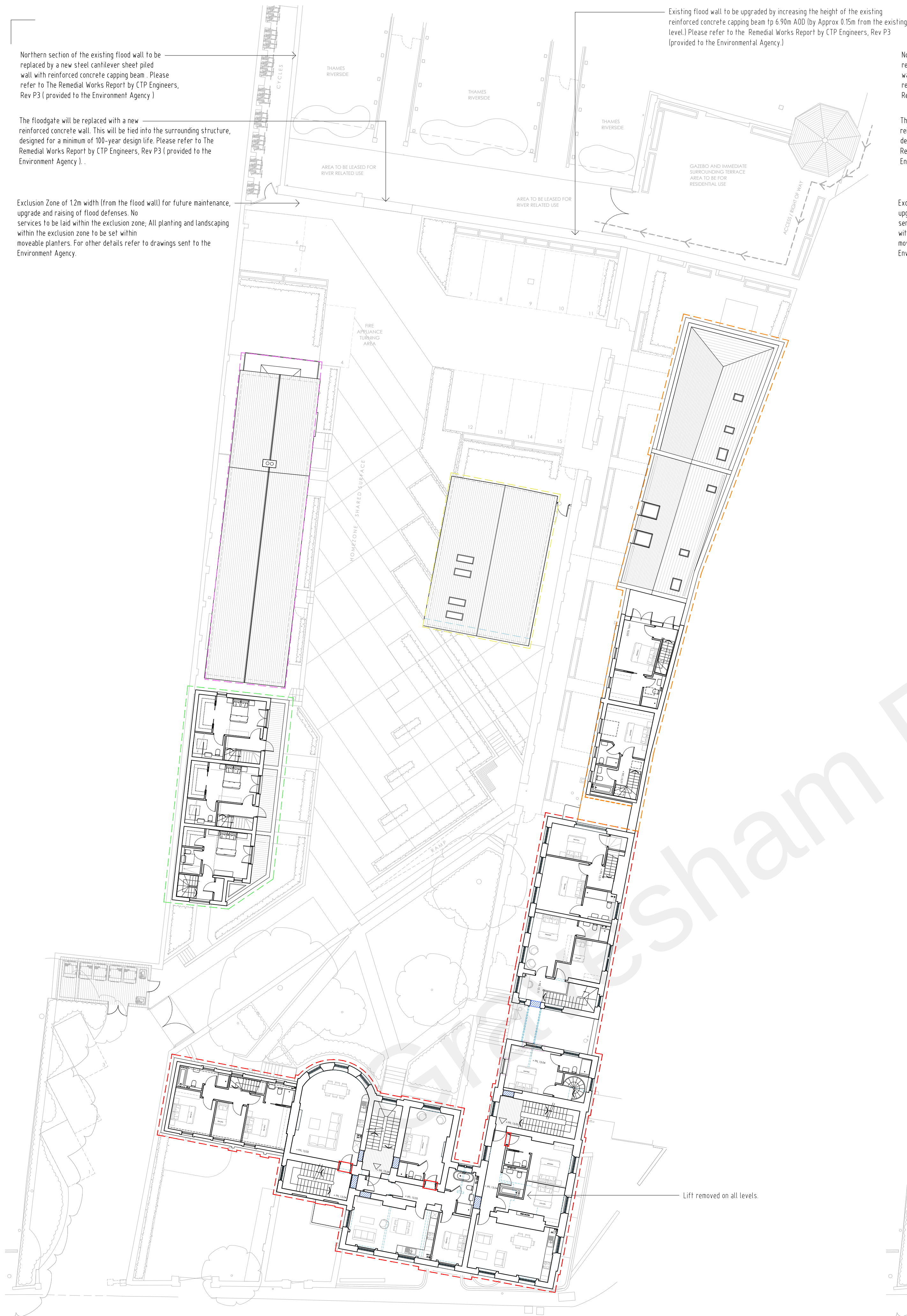
Proposed Site and First Floor Plan
