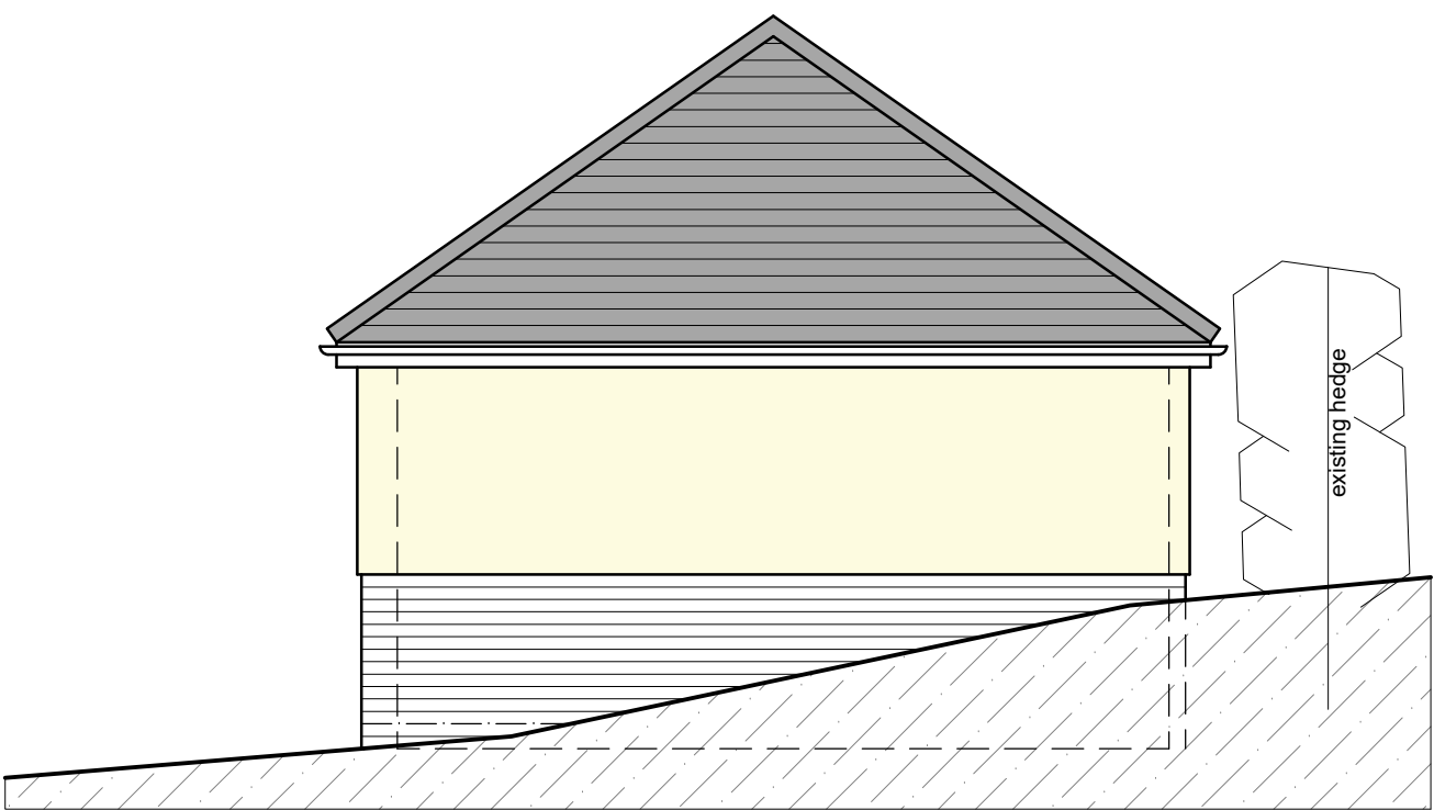
SIDE ELEVATION (1:50)
