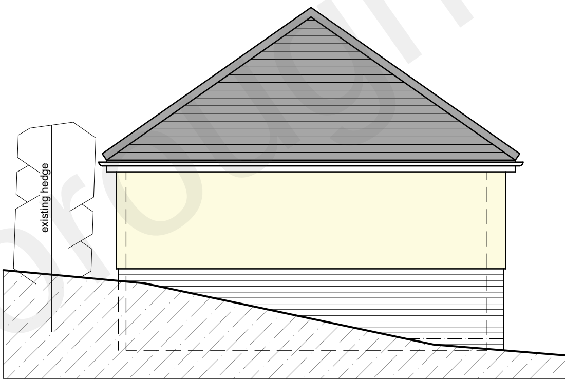
SIDE ELEVATION (1:50)
