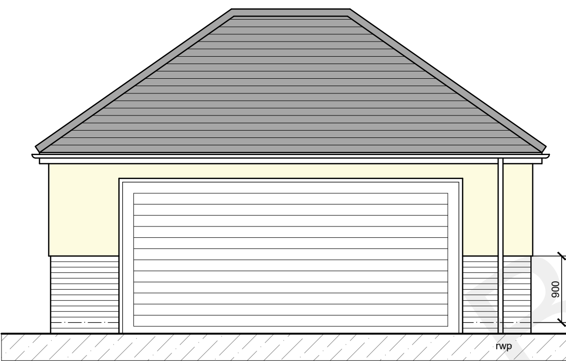
FRONT ELEVATION (1:50)
