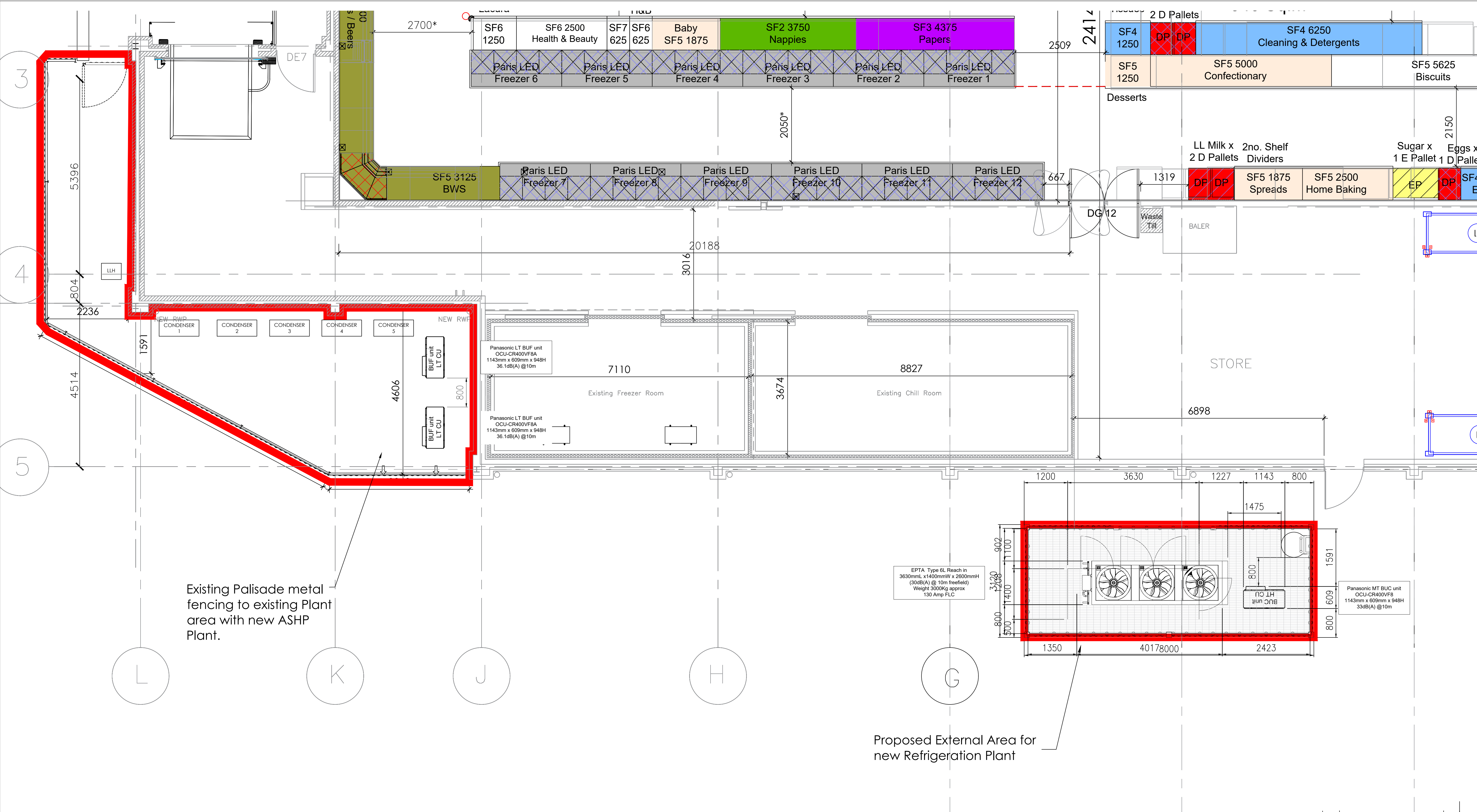
PROPOSED PLANT AREA - SCALE 1:50
